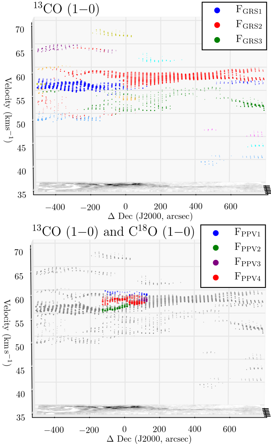
Figure 9. Shown are position-position-velocity diagrams covering the large-scale region surrounding Cloud F. The upper panel displays the Gaussian decomposition results for the ^{13}\text{CO} (1 – 0) GRS observations, where the colour of each point represents its association with a coherent velocity component (see Appendix E). The three most extended components are shown in the legend in the upper right of the panel. The lower panel displays the same position-position-velocity diagram with the GRS observations shown in grey, overlaid with the structures determined from the IRAM-30m \text{C}^{18}\text{O} (1 – 0) observations shown in colours identical to Figure 6 (see legend in upper right of panel). The size of each point represents its relative peak intensity. The mass surface density map of Kainulainen & Tan (2013) is shown on the base of each plot. Note, the coordinate offsets of these plots are relative to the centre of the mapped region: RA (J2000) = 18^{\text{h}}53^{\text{m}}19^{\text{s}} , Dec (J2000) = 01^{\circ}27'21'' ( l = 34.441^{\circ} , b = 0.247^{\circ} ).
