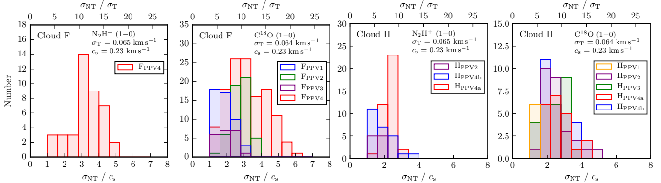
Figure 8. Cloud F (left two panels) and Cloud H (right two panels) histograms of the non-thermal contribution to the velocity dispersion over the gas sound speed (lower axis on each plot; c_s = 0.23 \text{ km s}^{-1} at 17 K, given a mean molecular weight of 2.33 a.m.u). The upper axis labels on each plot show the non-thermal contribution to the velocity dispersion over the thermal contribution to the velocity dispersion, where \sigma_T = 0.065 \text{ km s}^{-1} and 0.066 \text{ km s}^{-1} , for \text{C}^{18}\text{O} (30 a.m.u) and \text{N}_2\text{H}^+ (29 a.m.u), respectively. Colours represent the various velocity components (see Figures 6 and C3).
