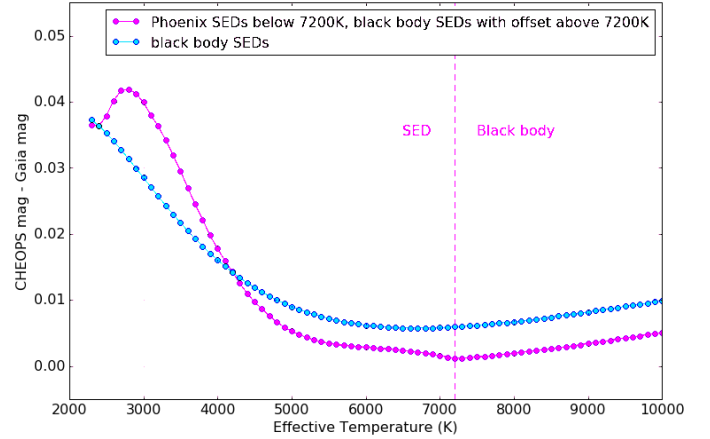
Fig. B.1. Difference between the CHEOPS magnitude and Gaia magnitude, X - G , as a function of the effective temperature of the star, using a SED for stars with T_{\text{eff}} < 7200\text{K} and the black body spectral distribution for T_{\text{eff}} > 7200\text{K} (magenta curve). The blue curve shows the same but always uses the black body approximation.
