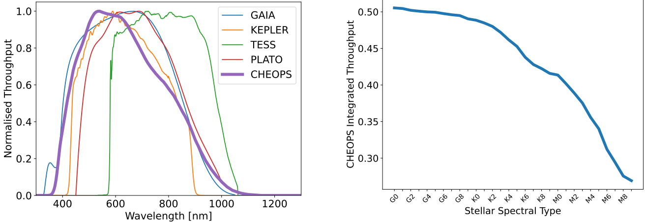
Fig. 3. CHEOPS throughput. Left: normalised CHEOPS throughput as a function of wavelength. For comparison, normalised Gaia , Kepler , TESS, and PLATO throughput are also plotted. Note the similarity between CHEOPS and Gaia throughput. Right: CHEOPS integrated throughput as a function of the star’s spectral type using PHOENIX model for the SED (Hauschildt et al. 1999a,b). This represents the fraction of all incident photons in the 330 nm to 1100 nm wavelength range converted into photoelectrons.
