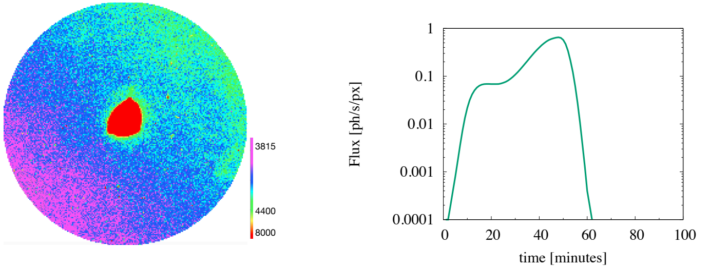
Fig. 24. Example of an image with high Earth's stray light contamination (visit ID: CH_PR300059_TG001201). Note the inhomogeneous background going from 3815 to 4400 ADUs. In cases like this, the background correction done by the DRP does not work properly. We recommend ignoring these images during the light curve analysis. The Earth's stray light contamination is a periodic function of the orbit, depending on the time and pointing. A simulation of stray light variation (normalised) during one orbit is given on the right.
