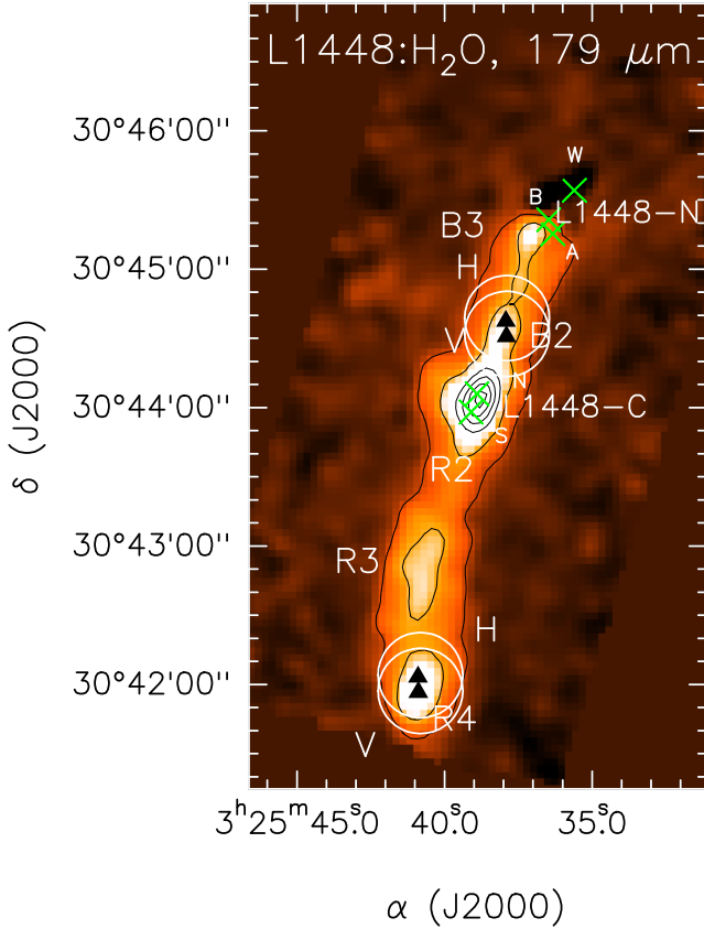
Figure 3. L1448 outflow and corresponding observed positions. The background image represent the H 2 O emission at 179 \mu m from the WISH program (Nisini et al. 2013). The circles show the vertical (V) and horizontal (H) polarization HPBW at the observed positions, whose centres are indicated by the triangles. The green crosses indicate the positions of the millimetre continuum sources (N, S, A, B, and W; Kwon et al. 2006).
