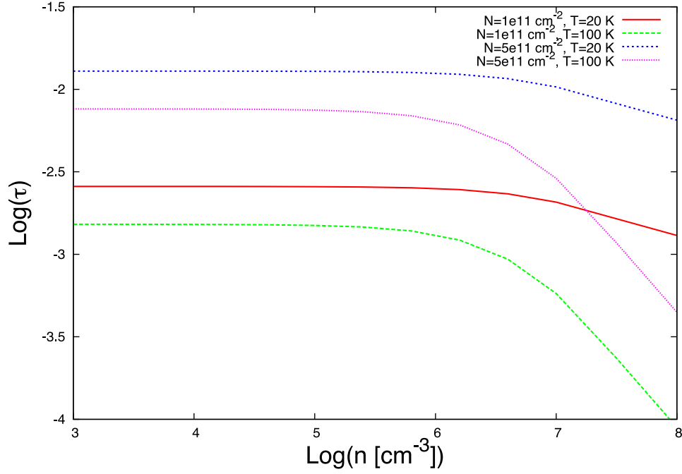
Figure B1. o- \text{NH}_3 ( 1_0-0_0 ) opacity as a function of \text{H}_2 particle density, from LVG calculations using RADEX. The different curves show different values of column density and kinetic temperature. Linewidth used in all cases is 10 \text{ km s}^{-1} (average observed linewidth).
