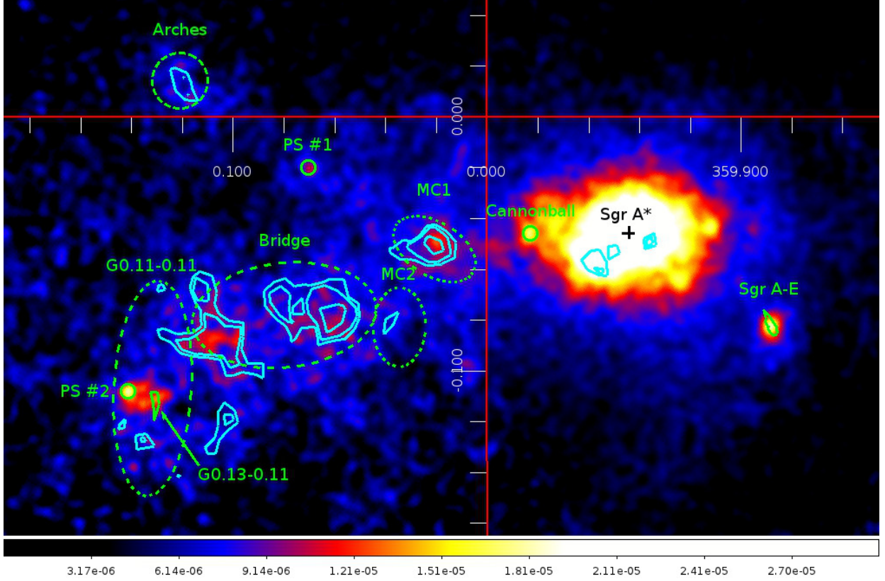
Figure 3. NuSTAR 10-20 keV exposure-corrected smoothed image of the GC region in the Galactic coordinates [ ^{\circ} ]. Green dashed ellipses: selected molecular clouds. Cyan contours: 6.4 keV Fe K \alpha continuum-subtracted intensity contours from XMM-Newton . Green polygons: Chandra morphologies of the two X-ray filaments detected above 10 keV. Green circles ( r = 10'' ): two hard X-ray point sources. PS #1 and #2 are known Chandra point sources, CXOUGC J174551.9–285311 and CXOUGC J174622.7–285218, respectively (Muno et al. 2009).
