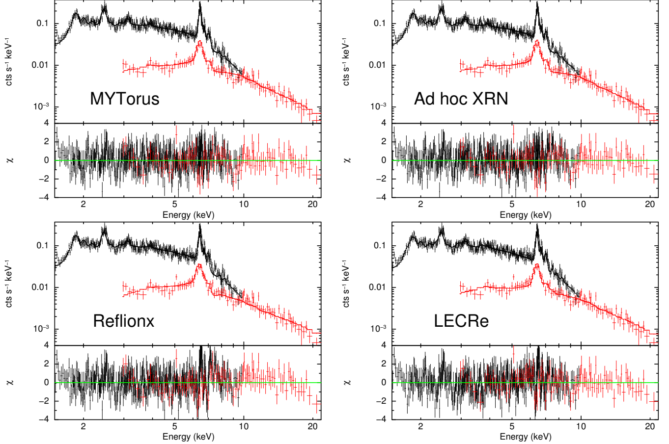
Figure 10. 1.5–20 keV XMM-Newton (black) and NuSTAR (red) spectra of the Bridge fit with the MYTorus (upper left), ad hoc XRN (upper right), reflionx (lower left) and LECRe electron model (lower right).
