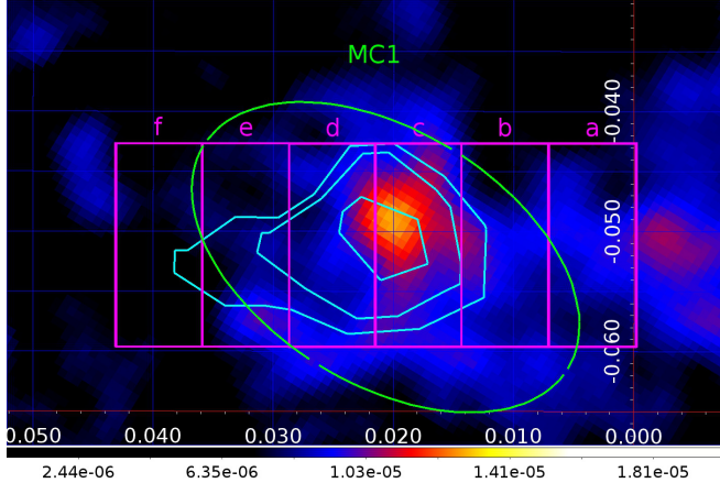
Figure 4. NuSTAR 10-20 keV image zoomed around MC1 cloud region in the Galactic coordinates [ ^{\circ} ] overlaid with a region used for extracting XMM-Newton and NuSTAR spectra of MC1 (green), Fe K \alpha line intensity contours from 2012 XMM-Newton observations (cyan), and the six 26'' \times 61'' rectangular subregions (magenta) defined in Clavel et al. (2013).
