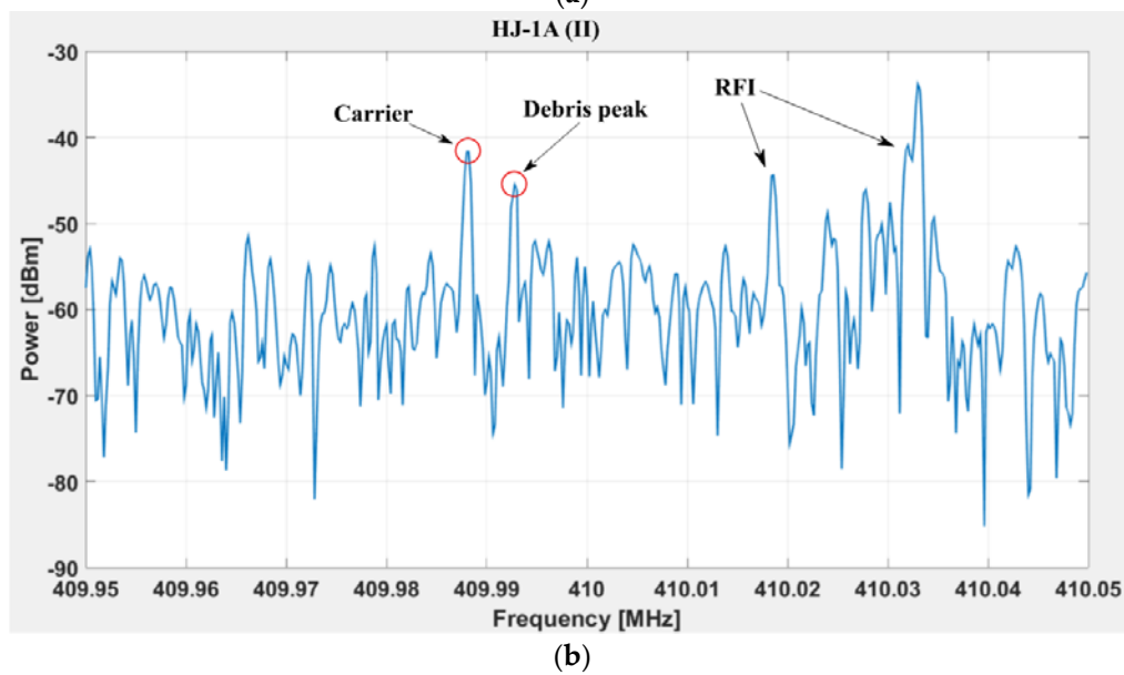
Figure 6. Debris HJ-1A (second passage): (a) spectrogram; (b) screenshot of the spectrum analyzer at the center of the visibility interval (Table 4).
