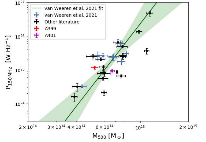
Fig. 9: Mass and radio power relation. The fitted regression line with a 3\sigma confidence interval in the shaded area and the data points in cyan come from the sample in van Weeren et al. (2021) . The literature data points in black are taken, similar to van Weeren et al. (2021) , from previous LOFAR and GMRT studies, and a correlation line is fit using the bivariate correlated errors and intrinsic scatter (BCES) orthogonal regression algorithm ( Akritas & Bershady 1996 ). We left out the radio halo candidates. The radio halos A399 and A401 are added. Error bars include statistical and systematic uncertainties.
