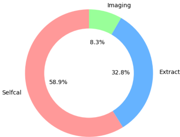
Fig. A.1: CPU core hours in percentage from the total amount for self-calibration, extraction, and imaging for making the image from A399-401. This is based on the calibration of A399-401 with 24 boxes within 0.6 degrees from the pointing center.
