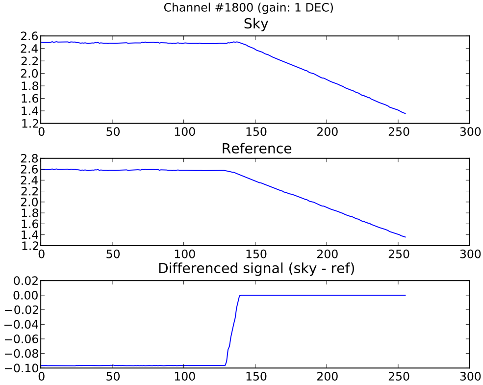
Figure 2: Example of the data acquired during the first calibration (channel #1800, gain state is 1 DEC). The average output voltage ( y ) is plotted against the raw DAE offset value ( x ). Note that for offsets smaller than \sim 130 DEC the output voltage after the digital-to-voltage calibration does not change (as the input voltage does not as well): this is the normal behavior. However, for offsets greater than 130 DEC the ADC saturates and therefore eq. (2) is adding an offset that is no longer the same used in eq. (1). This is most easily seen in the differenced data, which exhibit a sudden jump.
