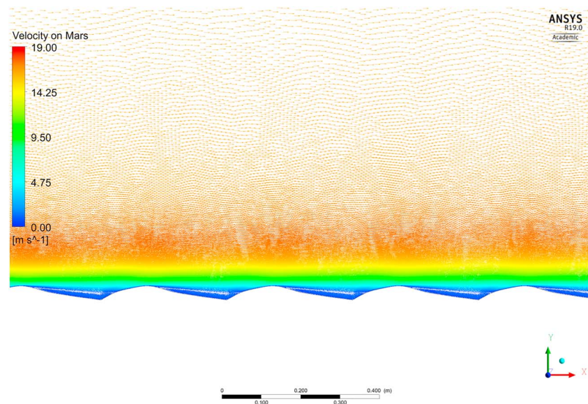
Figure 5. Wind velocity distribution over simulated ripples under Mars conditions for inlet velocities of 15 m/s. Note that the wind velocity is larger at the ripple crests. Vortices form between successive ripples, as shown more clearly in Figures 8b and 9b.
