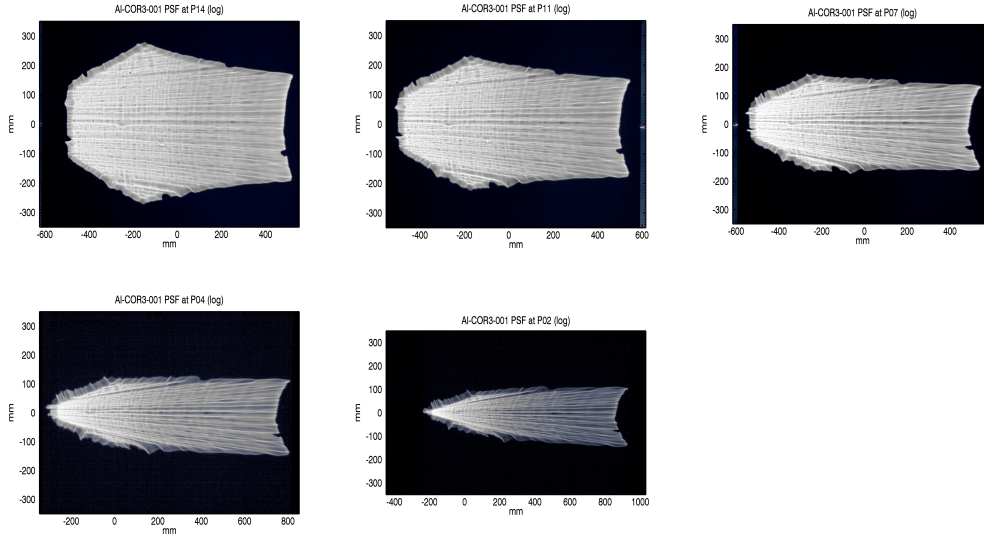
Figure 5. Image of the Pseudo-PSF of ASTRI-SST corona 3 segment acquired from the setup described in Fig.4: respectively from left to right dist_{scr-mirr} = 4761\text{ mm} , 5794\text{ mm} , 7059\text{ mm} on row 1, and dist_{scr-mirr} = 8183\text{ mm} , 8840\text{ mm} on row 2
