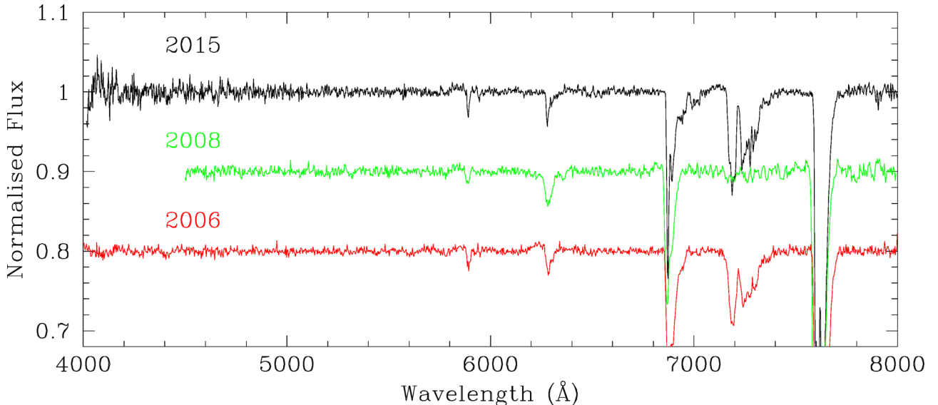
Figure 3. Comparison of the normalized spectra of S2 0109+22 taken in different epochs. From top to bottom: 2015 spectrum (SNR \sim 650); 2008 spectrum (SNR \sim 500) (Landoni et al. 2013); 2006 spectrum (SNR \sim 500) by (Sbarufatti et al. 2009). SNR estimated at 5500 Å for resolution element of 15 Å. The 2008 and 2006 spectra are shifted of 0.1 and 0.2, respectively.
