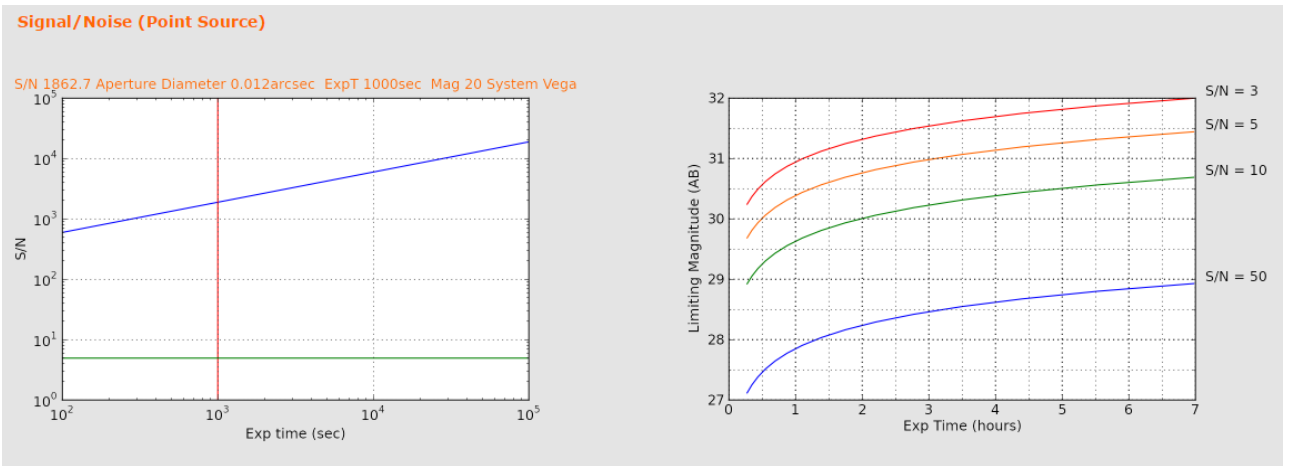
Figure 6. Plot the trend of the S/N against the exposure time for a wide range of integration times
