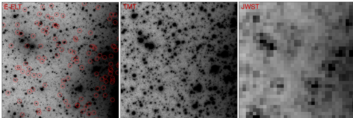
Figure 10. 1'' \times 1'' E-ELT (left), TMT (center), and JWST (right) images at 6 r_e from the centre of the 1 Gyr old NSC at 2 Mpc. In the left panel the red circles show J=28 mag stars, corresponding to the main-sequence turn-off magnitude.
