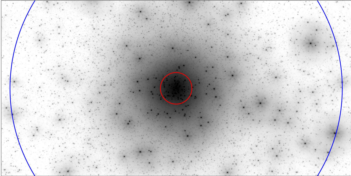
Figure 9. Zoom of a 6'' \times 3'' region of a J-band simulated with MICADO@E-ELT. The circles show effective radius ( 0''.27 , in red) and tidal radius ( 2''.85 , in blue) of the cluster.
