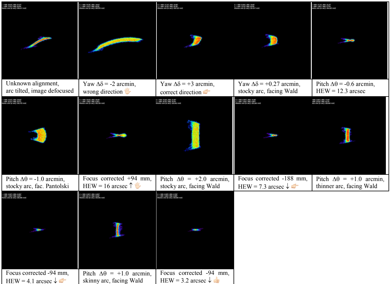
Figure 20: simulated alignment process with the parallel beam at 1.49 keV. The detector size is \frac{1}{4} of PIXI's.
