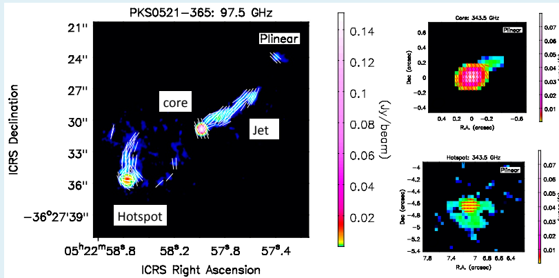
Fig. 2 Linear polarization emission (colours) and position angles (vectors) in ALMA Band 3 and 7 of PKS 0521-365
