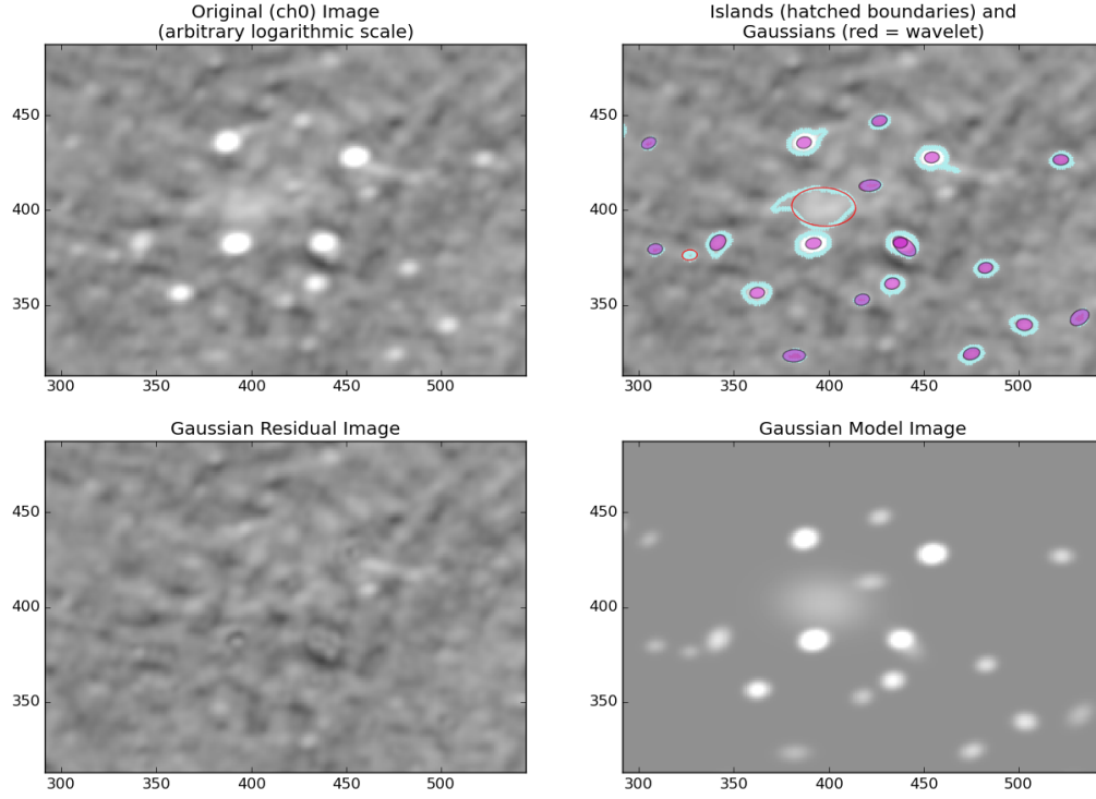
Fig. A.1. Output of the PyBDSM source finder tool. The axis units are in pixels. From left to right and from top to bottom : original image on which PyBDSM is run (in this example, the ID2 map of Table 3); islands of significant emission (cyan contours) and fitted Gaussians that model identified sources overlaid on the ID2 map; residual after the subtraction of the fitted sources; model of the reconstructed sky. The big red ellipse corresponds to the diffuse emission in the centre of the cluster.
