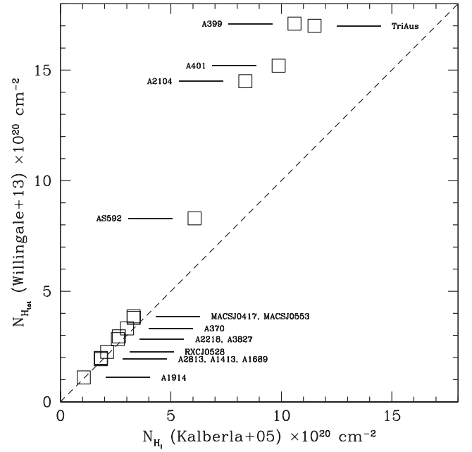
Figure 1. Comparison between the \text{H I} density column from Kalberla et al. (2005) and the total ( \text{H I} + \text{H}_2 ) density column from Willingale et al. (2013). The dashed line indicates the linear correlation as a reference.
