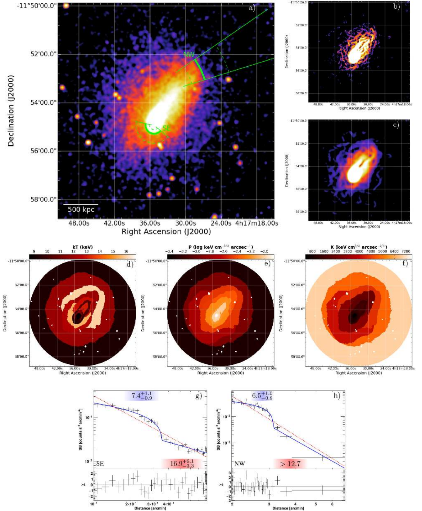
Figure 5. MACS J0417. The same as for Fig. 3. The goodness of fits is reported in Fig. C3. The positions of the edges are marked in green (cold fronts).
