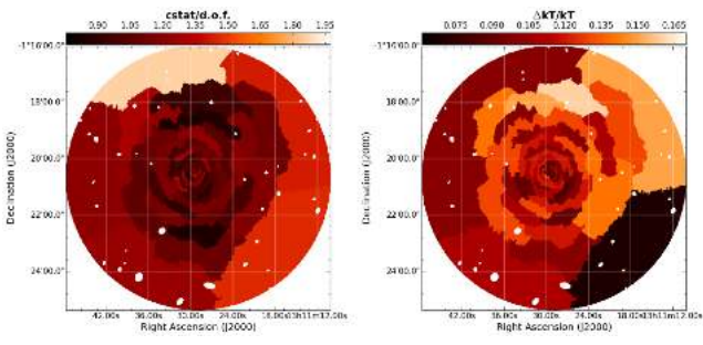
Figure C13. The same as Fig. C1, but for A1689 (cf. Fig. 16).
