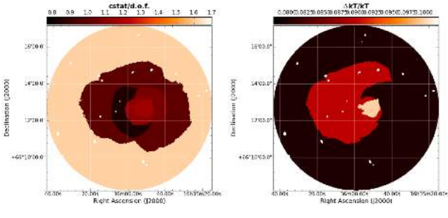
Figure C9. The same as Fig. C1, but for A2218 (cf. Fig. 11).
