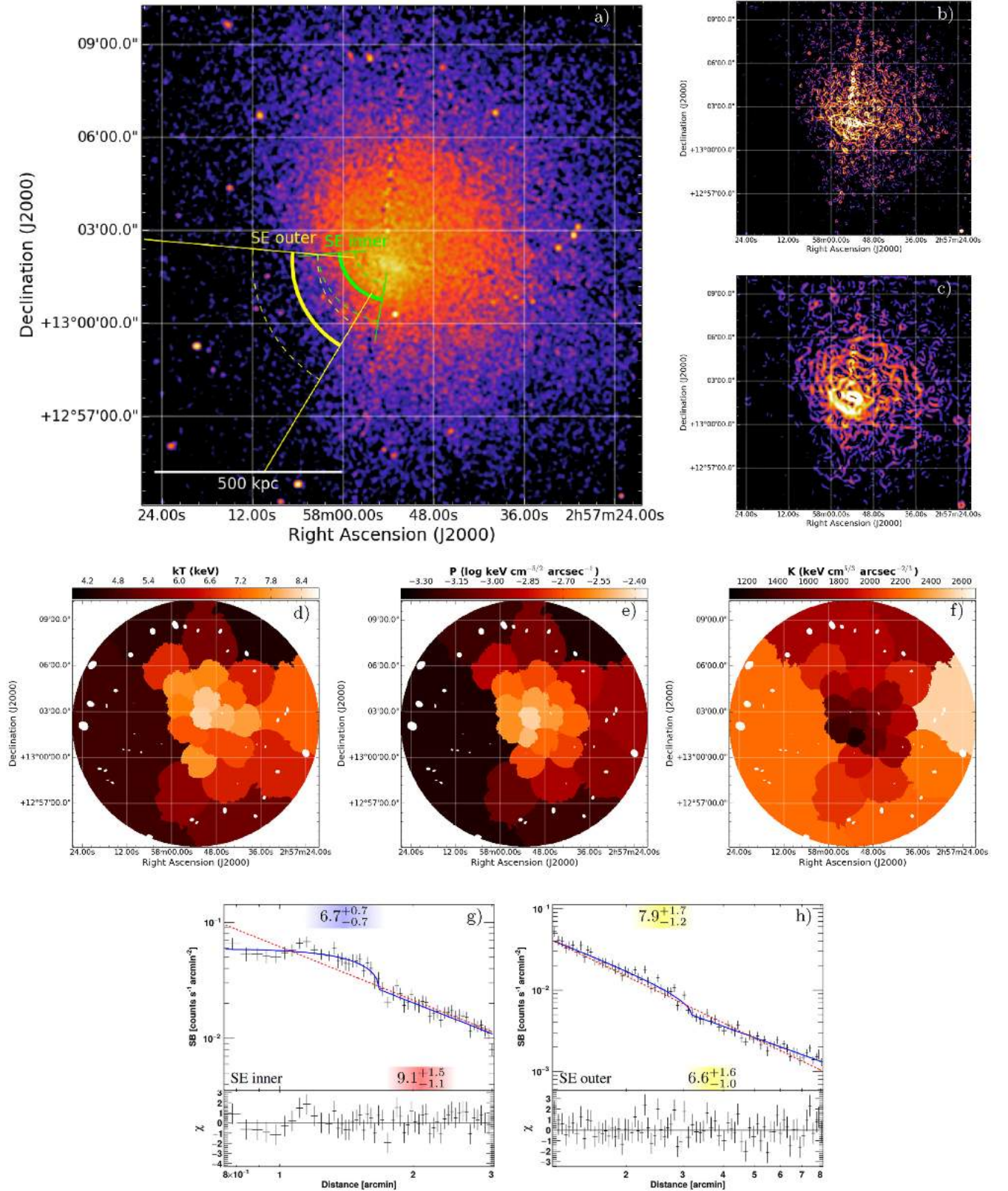
Figure 3. A399. Chandra 0.5–2.0 keV image (a), GGM filtered images on scales of 4 (b) and 8 (c) pixels, projected maps of temperature (d), pressure (e), entropy (f), and best-fitting broken power-law (solid blue) and single power-law (dashed red) models (residuals on the bottom) of the extracted SB profiles (g and h). The goodness of fits is reported in Fig. C1. The sectors where the SB profiles were fitted and the positions of the relative edges are marked in the Chandra image in green (cold front) and yellow. The dashed arcs show the radial limits used for measuring the temperature downstream and upstream the front, which values (in keV) are reported in the shaded boxes in the SB profiles. Note that in the GGM filtered images the straight and perpendicular features are artefacts due to chip gaps.
