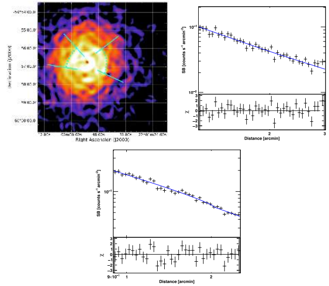
Figure D5. GGM filtered image of A3827 (the same as Fig. 17c) marked with the regions used to extract the SB profiles (left) and corresponding fits. The putative edge in the E sector is at r \sim 1.8 arcmin (right), whereas in the W sector is at r \sim 1.3 arcmin (bottom).
