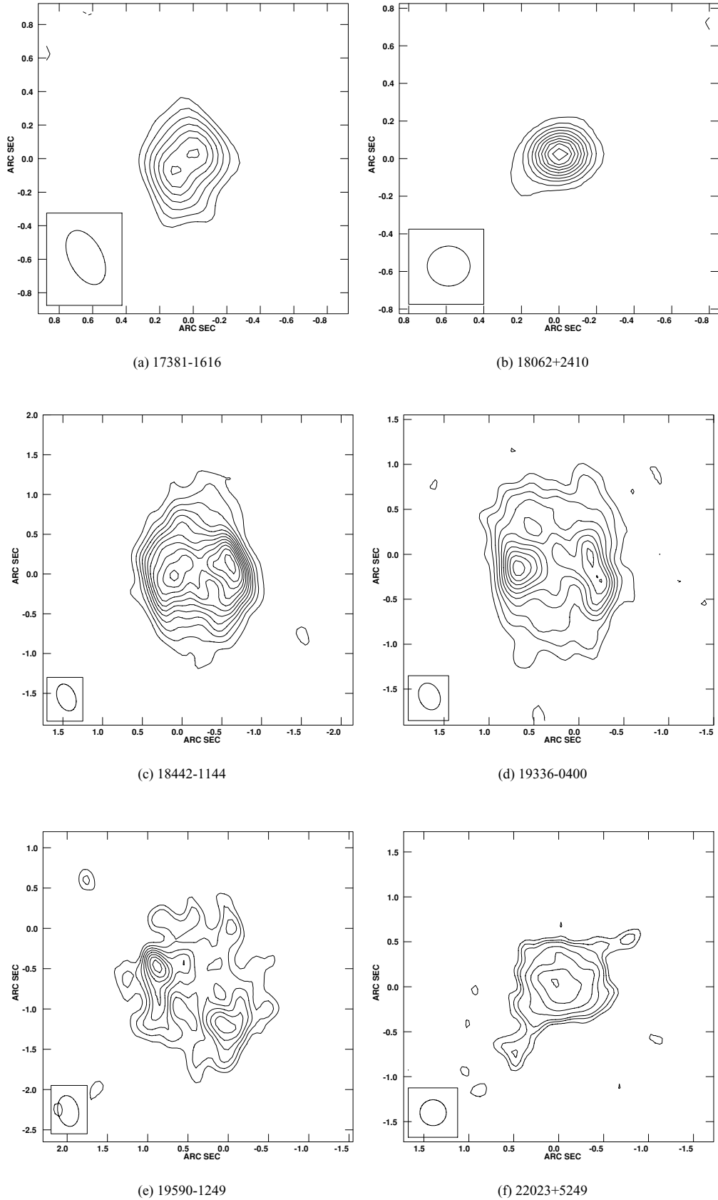
Figure 1. Radio maps at 8.4 GHz of the targets observed in high angular resolution. The flux density levels, in units of \mu\text{Jy beam}^{-1} , are: in 17381 (-3, 3, 4, 5, 6, 7, 8, 9)\sigma ; in 18062 (-3, 3, 6, 9, 12, 15, 18, 21, 24, 27, 30)\sigma ; in 18442 (-3, 3, 6, 9, 12, 15, 18, 21, 24, 27, 30, 33, 36)\sigma ; in 19336 (-3, 3, 5, 7, 9, 11, 13, 15, 17, 19, 21)\sigma ; in 19590 (-3, 3, 4, 5, 6, 7, 8, 9, 10)\sigma and in 22023 (-3, 3, 4, 5, 7, 9, 11, 13)\sigma ; where \sigma indicates the rms calculated in each map and listed in Table 2. The maps do not show any negative level, because no such levels are present in the mapped areas.
