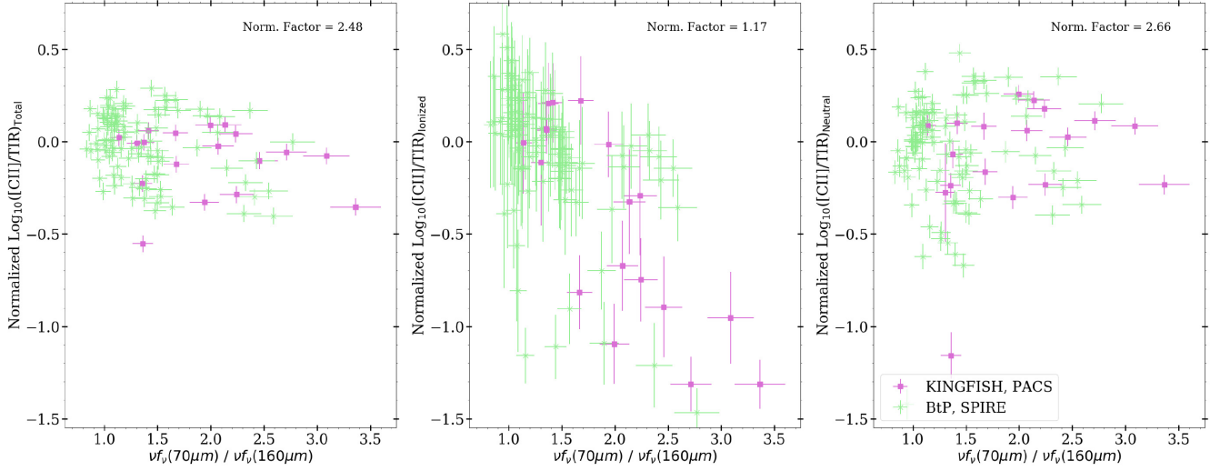
Figure 4. Left: The undivided [C II]/TIR measurements are plotted against \nu f_{\nu}(70\ \mu\text{m})/\nu f_{\nu}(160\ \mu\text{m}) flux ratios to show the moderate deficit behaviour observed in the galaxies in this sample. Middle: The isolated ionized phase [C II]/TIR measurements plotted against \nu f_{\nu}(70\ \mu\text{m})/\nu f_{\nu}(160\ \mu\text{m}) . Notice the steeper negative slope indicating the strong deficit behaviour in the ionized phase. Right: The isolated neutral phase [C II]/TIR measurements plotted against \nu f_{\nu}(70\ \mu\text{m})/\nu f_{\nu}(160\ \mu\text{m}) . No deficit behaviour is observed when only the neutral phase is considered. This builds on the work performed in Sutter et al. (2019). All [C II]/TIR ratios have been normalized by adding the absolute value of the average \log_{10}[\text{C II}]/\text{TIR} ratio for the given phase to highlight the different trends in each phase. For clarity, the normalization factors are seen at the top of each panel.
