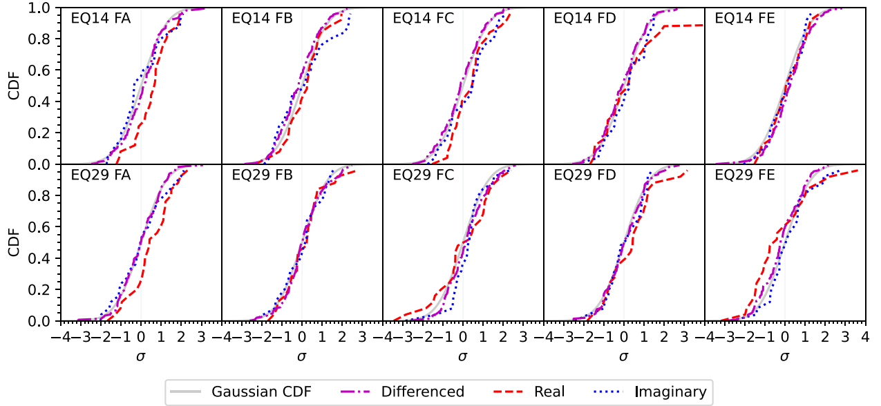
Figure 10. The cumulative distribution functions of the cross-power spectra at |\kappa_{||}| > 1.0 ‘pseudo’ h \text{ Mpc}^{-1} . The red dashed and the blue dotted lines show the CDFs of the real and imaginary parts of the power spectra, respectively, while the magenta dash dotted line shows the CDF of the noise realization obtained by differencing closure phases with the same underlying sky signal. As a reference, we also plot a Gaussian CDF with the same variance as the noise (grey solid line). The abscissa is given in units of standard deviations of the differenced closure phases.
