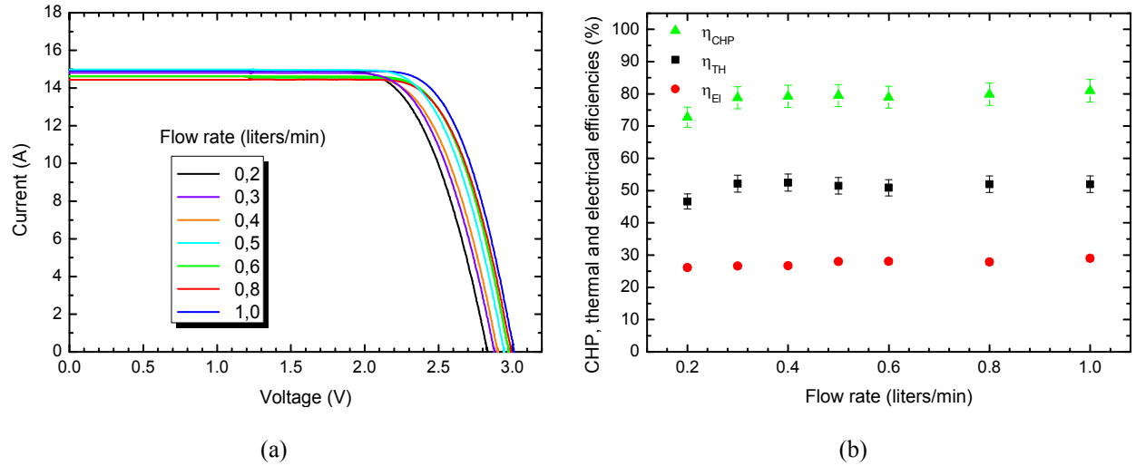
FIGURE 2. Flow rate dependence of the CHP performance under a DNI of 650 \text{ W/m}^2 . (a) IV curves obtained with different flow rates ranging from 0.2 to 1.0 liters/min and at T_{in} = 25^\circ \text{C} . (b) Electrical, Thermal and Total CHP efficiencies as a function of the flow rate.
