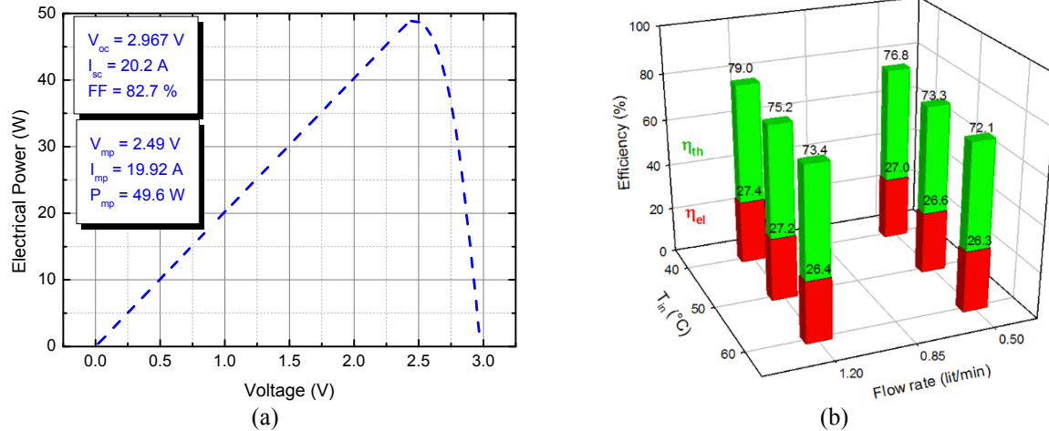
FIGURE 4. (a) PV curve obtained under a DNI of 900 \text{ W/m}^2 with a flow rate of 1.2 liters/min and inlet temperature of 40^\circ \text{C} . (b) Electrical (red), Thermal (green) and Total CHP efficiencies as a function of T_{in} and \dot{V} ; for each bar we indicate the values of electrical and total efficiencies.
