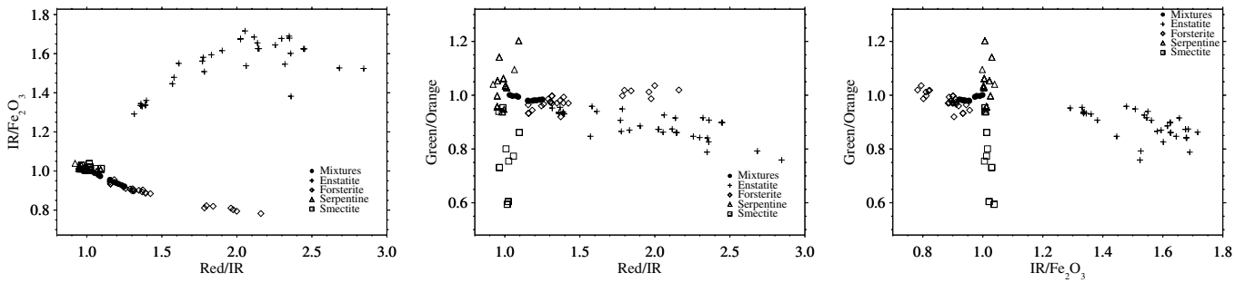
Fig. A.3. Defined ratios for RGB images together with mixtures.
