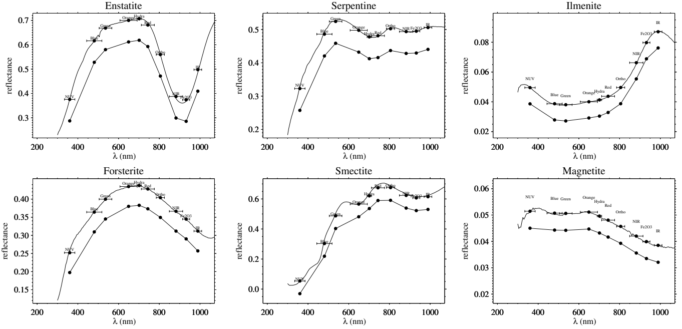
Fig. 1. Absolute spectra of anhydrous silicates (enstatite, forsterite) in the left panel , hydrated silicates (serpentine, smectite) in the middle panel , and oxides (ilmenite, magnetite) in the right panel as they would be observed through the full set of OSIRIS NAC filters. The solid lines above are laboratory data of the corresponding mineral with the central wavelengths of the NAC filters (dots) including their bandwidths (horizontal bars), while resampled laboratory data are arbitrarily (lowered by 1/8 compared to the maxima) offset for display.
