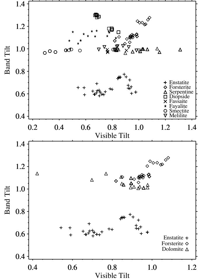
Fig. 3. Separation of minerals using visible tilt and band tilt.
