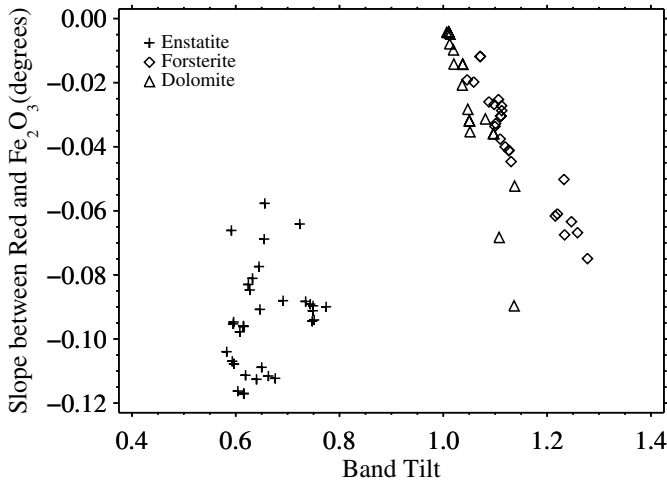
Fig. 6. Separation of minerals: slopes between the red and Fe 2 O 3 filters.
