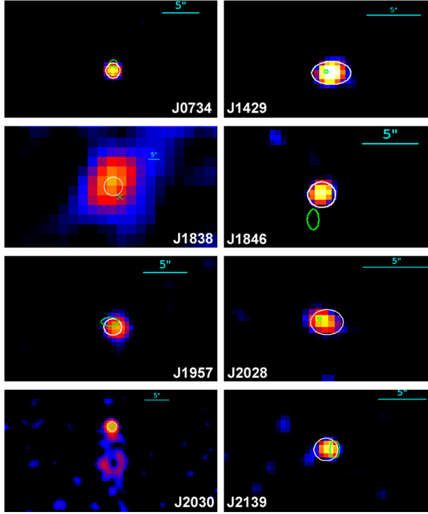
Figure 1. Chandra and XMM-Newton images of the pulsars listed in Table 1, taken in the 0.3–10 keV energy range. For a better visualization, we applied a Gaussian filter with a kernel radius of 3''. In each panel, the best-fit X-ray position (90% confidence errors) is shown by the white circle and the LAT \gamma -ray timing position ( 1\sigma errors) by the green ellipses. The latter are taken from the most recent compilation of the LAT \gamma -ray Pulsar Timing Models. The position of PSR J1838–0537 is taken from Pletsch et al. (2012a), where the positional error is not reported, and is marked by the green cross.
