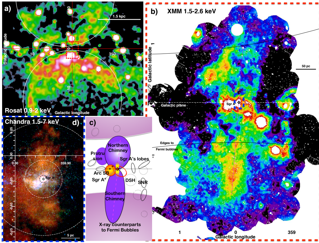
Figure 5: ( Panel a ) ROSAT (0.9-2 keV energy band) large scale map of the GC. The X-ray counterparts of the Fermi bubbles are strong X-ray emitters. The edges (white ellipses) are clearly detected on scales of several degrees, while they become confused (because of the short exposure of 200-300 s and soft X-ray energy band) close to the plane. The red dashed line indicates the XMM-Newton area covered by our survey. ( Panel b ) XMM-Newton map zooming into the central degrees of the Milky Way. The magenta dashed line intersects both Chimneys, passing through Sgr A*. The map shows the X-ray emissivity within the 1.5-2.6 keV energy band (see Fig. 4). ( Panel c ) Schematic view of the main diffuse X-ray emitting features within the central \sim 500 pc from Sgr A*. The red star and the yellow ellipses indicate the position of Sgr A* and of Sgr A's \pm 15 pc bipolar lobes. The large violet ellipses indicate the location and extension of the X-ray counterpart of the GCL with shell like morphology (northern Chimney), of its eastern protrusion and of its roughly symmetric southern counterpart (southern Chimney). The orange filled ellipse, the two red circles and the red ellipse indicate the location of the Arc super-bubble, the Quintuplet and Arches clusters and the super-bubble candidate G359.77-0.09 7 . The pink regions indicate the location of the edges to the Fermi bubbles. The dotted circles and solid ellipses indicate the position of bright X-ray sources with intense dust scattering halos and known supernova remnants. ( Panel d ) Chandra RGB map zooming into the central tens of parsecs of the Galaxy. The \pm 15 pc lobes are clearly visible in orange colour. The dashed circles have radii of 1, 5, and 15 pc.
