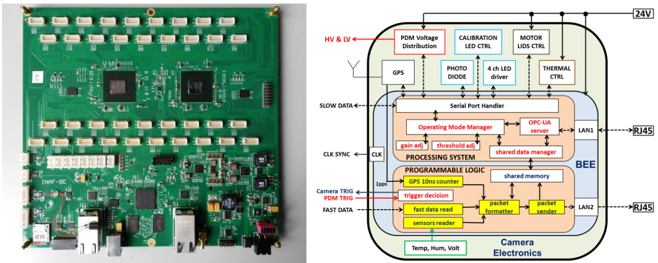
Figure 7. Left : The Back End Electronics. The board dimensions are 220mm x 250mm. Right : Block diagram of the BEE showing the architecture designed for ASTRI SST-2M as implemented inside the Zynq FPGA. The ancillary subsystems controlled by the BEE are also highlighted. On the left, there are the signals that interface each PDM. On the right, there are the LAN links that allows the communication to the external world: the Camera Control and the Camera Server.
