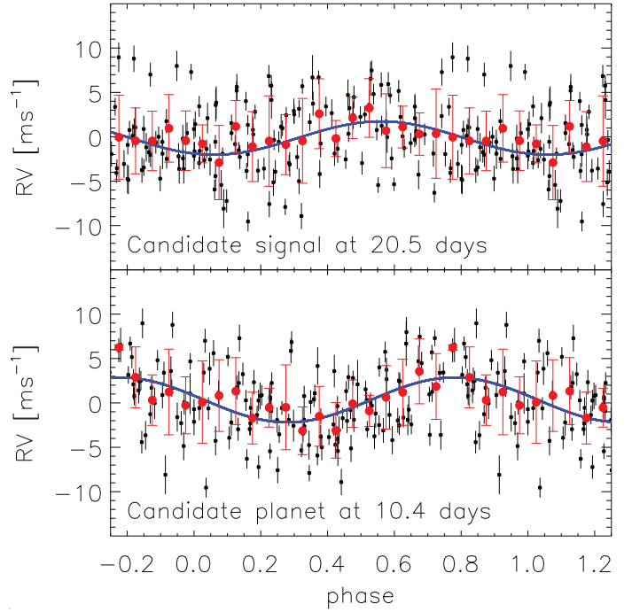
Fig. 13. Residuals and errors of the RVs in black dots folded to a period of 20.5 (top panel) and 10.4 days (bottom panel) with semi-amplitudes of 1.88 and 2.52 m s -1 , respectively. We used the data after pre-whitening the 16.3-day signal (top) and the 16.3- and 6.9-day signal (bottom) using the MA method. The red dots correspond to averages in 0.05 phase intervals. We show the best sinusoidal fits in blue.
