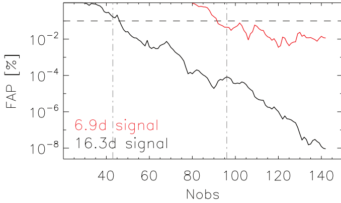
Fig. 5. FAP development for the 16.3-day (black) and the 6.9-day (red) signals of the RV data using an increasing number of data points. The dashed horizontal line shows the analytical 0.1% FAP level, and the two vertical dash-dotted lines divide the data into the different seasons.
