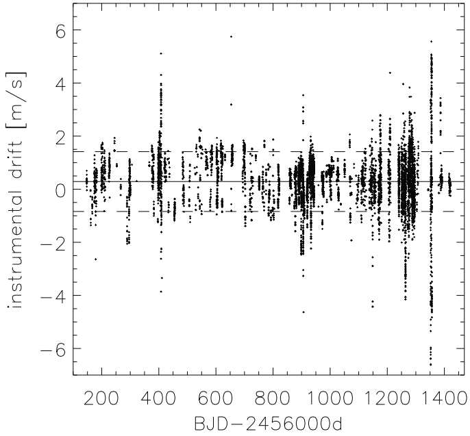
Fig. 1. All available 8199 instrumental drifts distributed over 356 nights. The solid line indicates the mean value and the dashed lines the 1\sigma interval.
