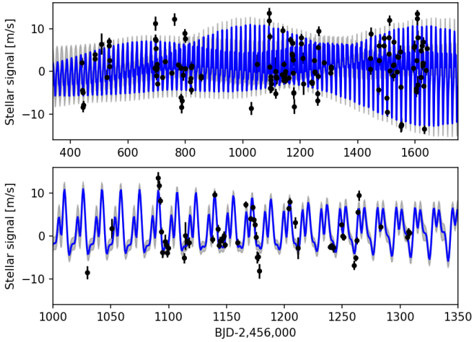
Fig. 11. Radial velocity residuals time series (black dots) after subtracting our best-fit orbital solution for GJ 3942 b. The blue line with gray shaded 1\sigma regions represents our best-fit GP quasi-periodic model for the correlated stellar noise. The top plot shows the complete dataset, while the lower plot shows a blow-up of the third epoch for easier visualization of the agreement between the model and the data.
