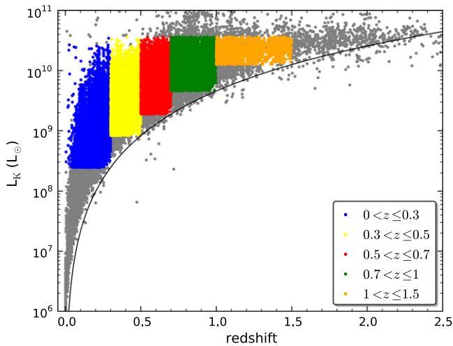
Figure 2. K -band luminosity vs. redshift for the selected sample of low-mass galaxies ( 10^7 \leq M_* \leq 3 \times 10^9 M_\odot ). The solid black line represents the K -band sensitivity limit of 23 mag. The color-coded regions show the complete redshift bins considered in the stacking analysis.
