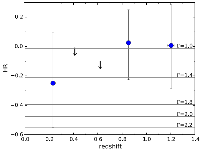
Figure 7. Hardness ratio vs. redshift for the five complete redshift bins. The lines indicate the HR from a population of XRBs with \Gamma = 1, 1.4, 1.8, 2, 2.2 (from top to bottom) and Galactic N_H .
