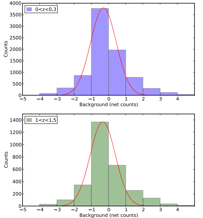
Figure 4. Background net count distribution for randomly distributed source positions in the 0 < z < 0.3 (top) and 1 < z < 1.5 (bottom) redshift bins. The red solid line shows the fit of a Gaussian distribution with offset = -0.295 and \sigma = 1.052 for the 0 < z < 0.3 bin and offset = -0.334 and \sigma = 1.037 for the 1 < z < 1.5 bin.
