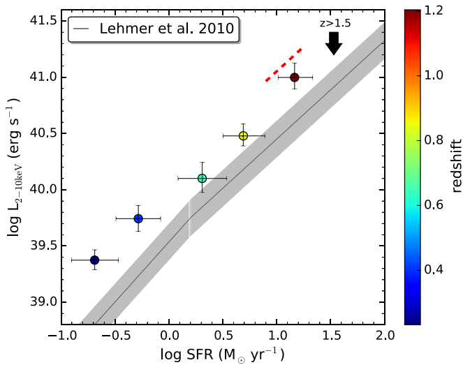
Figure 5. Luminosity (2–10 keV) vs. average SFR of each stacked redshift bin for the sample of starburst and late-type dwarf galaxies. The gray line shows the L_{\text{XRB}}-M_* -SFR correlation for XRBs from Lehmer et al. (2010) with a scatter of 0.34 dex. The 1\sigma error bars account for the stacking uncertainties and the statistical errors on the SFRs and M_* . The red dashed line indicates where the expected contribution from XRBs would lie if the metallicity were a factor three lower than the solar one at z > 1 as predicted by Fragos et al. (2013).
