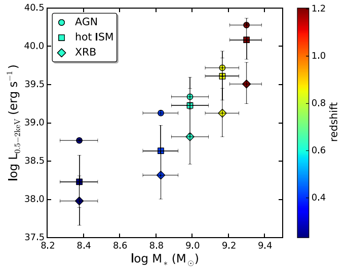
Figure 6. Nuclear X-ray luminosity (circles), hot ISM luminosity (squares) and XRB luminosity (diamonds) in the (0.5\text{--}2\text{ keV}) band vs. average stellar mass of each stacked redshift bin.
