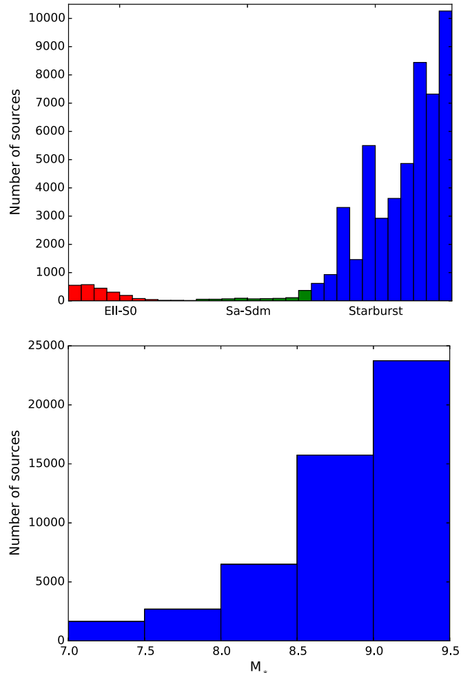
Figure 1. Top: distribution of morphologies for the sample of low-mass galaxies. Early-type galaxies are shown in red, spiral galaxies in green, starburst in blue. Bottom: distribution of stellar masses for the sample of non-elliptical dwarf galaxies.
