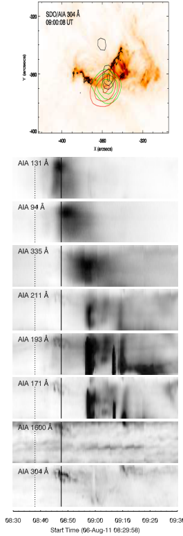
Fig. 5 SOL20110806. top : SDO/AIA 304 Å image acquired at around 09:00 UT (reverse intensity scale), with overplotted RHESSI emission contours from simultaneous observations: 3-6 keV (red), 6-12 keV (green), and 25-50 keV (black). The black contours represent the SST Ca II H emission. The extruding structure is the region between -400 and -300 [x-coordinate] and -360 [y-coordinate]; bottom : SDO/AIA intensity time slices along the extruding structure for different wavelengths. The bottom of each panel corresponds to the easternmost part of the extruding structure, the top to the part closest to the \delta -spot. The dotted vertical lines indicate the start of the flare according to the HXR emission; the solid vertical lines, the flare peak (adapted from Guglielmino et al. 2016)
