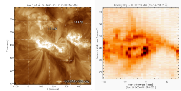
Fig. 6 SOL20120309. Left : AIA/SDO 193 Å image of AR NOAA 11429 acquired at 22:00:57 UT, showing the coronal configuration of the active region; right : EIS/Hinode intensity map acquired in the line Fe XIV 264.700 Å (reverse color) during the flare occurrence. The brightest pixels indicate the location of the footpoints.
