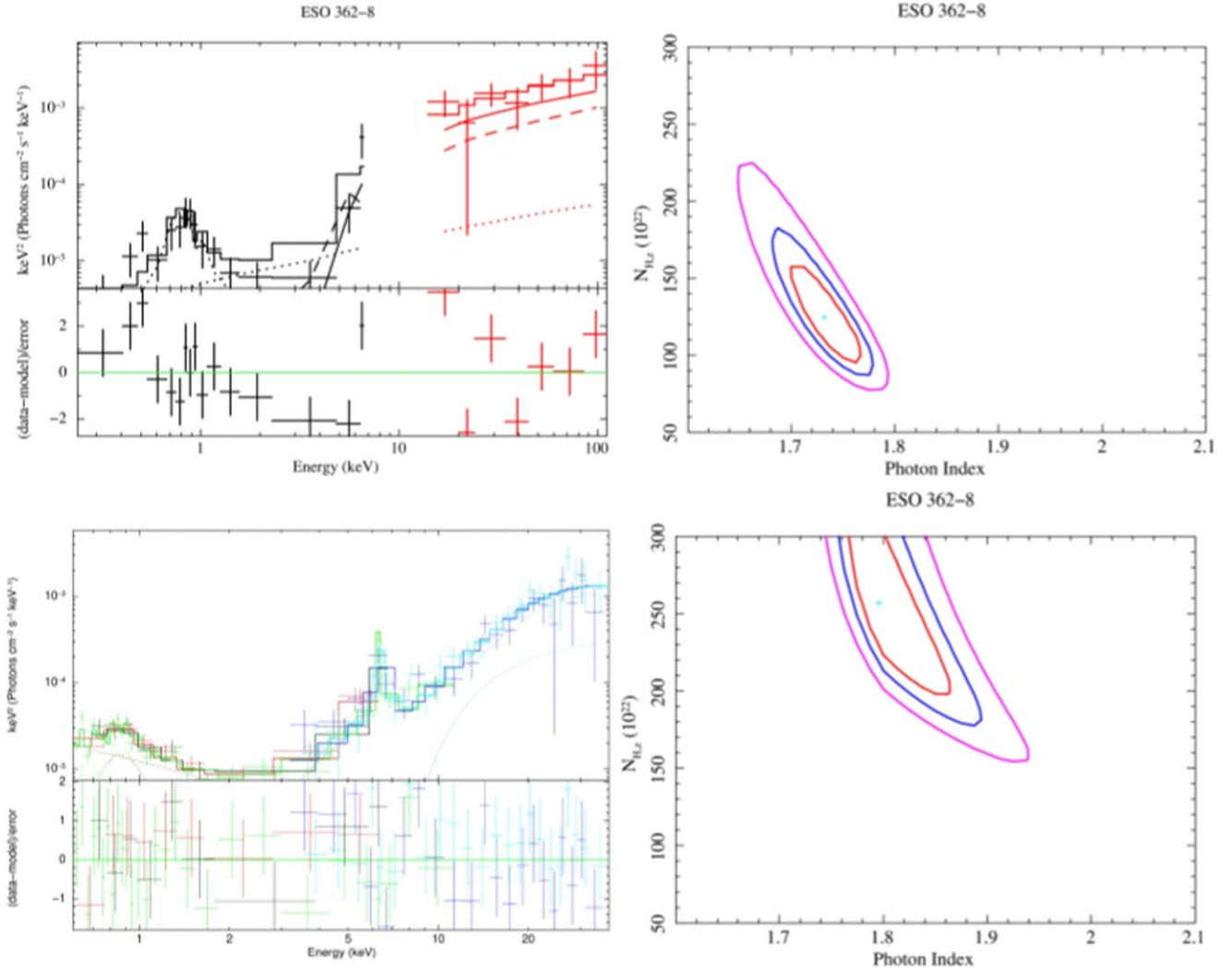
Figure 3. Top: the borus02 fit for the archival XMM-BAT data of ESO 362–8 with the contours of N_{H,l.o.s.} ( \times 10^{22} \text{ cm}^{-2} ) vs. photon index. The contours represent the 68%, 90%, and 99% confidence levels. Bottom: the borus02 fit of the NuSTAR–XMM-Newton data alongside its contour of the same parameters.
