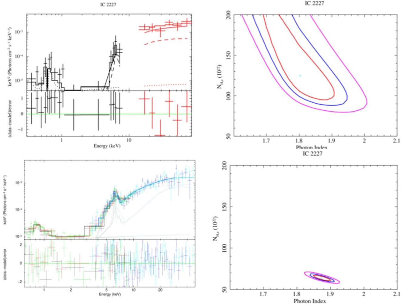
Figure 4. Top: the borus02 fit for the archival XRT-BAT data of IC 2227 with the contour of N_{\text{H,I.O.S.}} (\times 10^{22} \text{ cm}^{-2}) vs. photon index. The contours represent the 68%, 90%, and 99% confidence levels. Bottom: the borus02 fit of the NuSTAR–XMM-Newton data alongside its contour of the same parameters.
