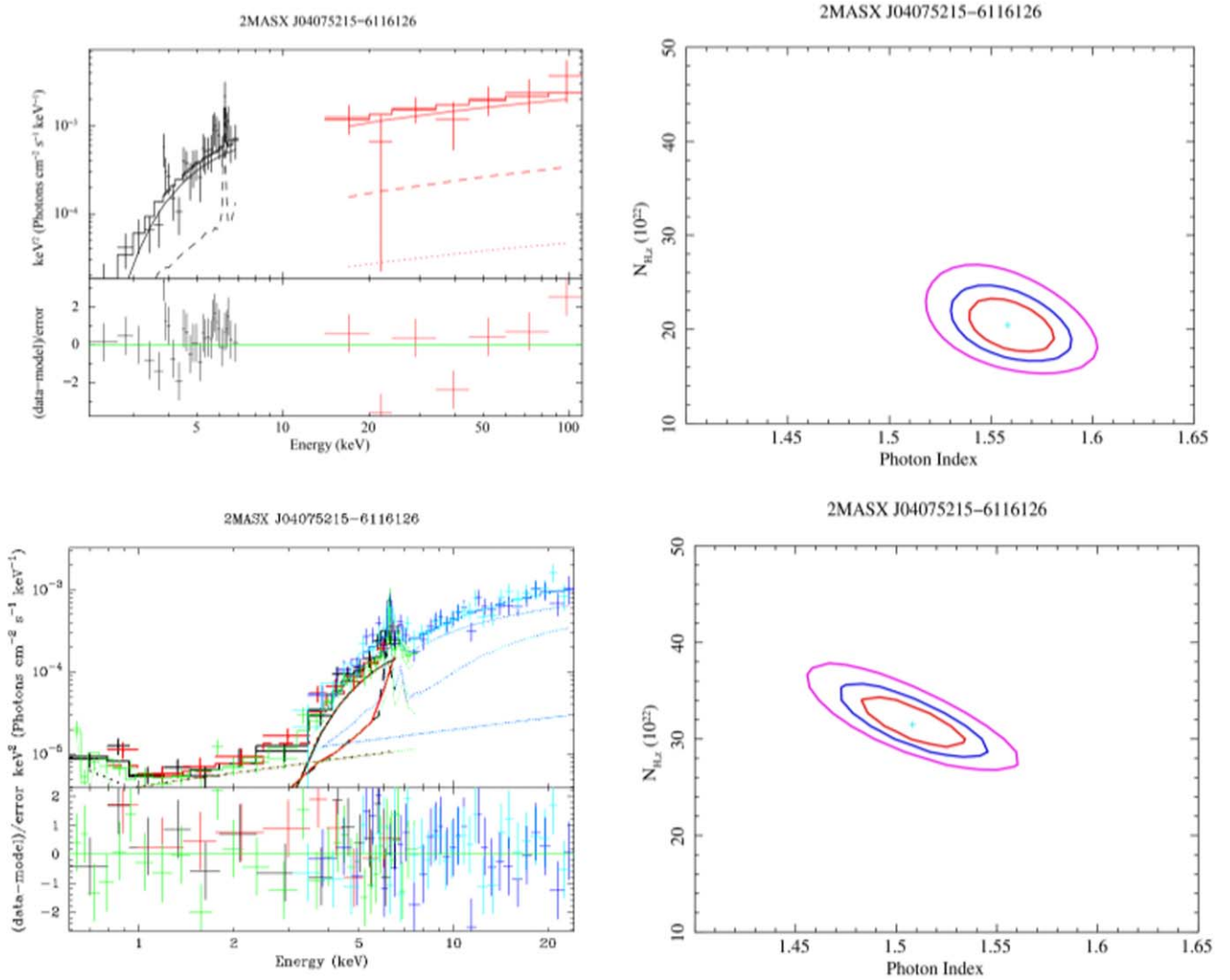
Figure 2. Top: the borus02 fit for the Chandra-BAT data of 2MASX J04075215–6116126 presented in S22 with the contours of N_{H,Lo.s.} ( \times 10^{22} \text{ cm}^{-2} ) vs. photon index. The contours represent the 68%, 90%, and 99% confidence levels. Bottom: the borus02 fit of the NuSTAR–XMM-Newton data alongside its contour of the same parameters.
