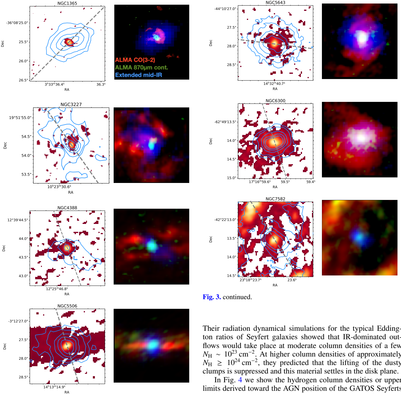
Fig. 3. Galaxies with extended mid-IR emission. Left panels: in color are the ALMA MSF 870 \mu\text{m} continuum images (with both the unresolved and the extended emission) from GB21. The blue contours are the mid-IR PSF-subtracted images with the same levels as in Fig. 2. The FoV is 2'' \times 2'' . We also plot with the dashed lines the approximate PA of the ionization cones, NLR and/or outflows (see Sect. 3.4). Right panels: RGB images constructed with the ALMA CO(3–2) image (red), ALMA 870 \mu\text{m} continuum (green), and extended mid-IR emission (blue). The FoV is approximately the same as in the left panels.
