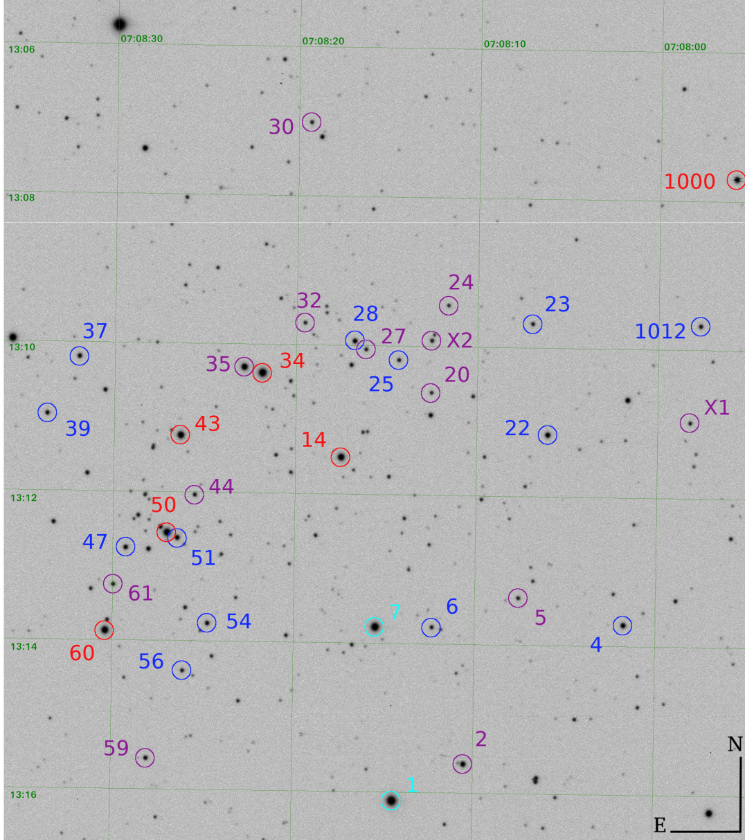
Fig. 2. Finding chart of core of NGC 2345, black square in Fig. 1. The image is one of our V-band frames and covers a region of sky around 10' \times 11' . Stars for which we have spectra are inside circles of different colours according to their spectral types, as explained in the text, to facilitate its identification. Stars X1 and X2, identified as Be stars by Mathew & Subramaniam (2011), without WEBDA numbering, are also included. North is up and east is on the left.
