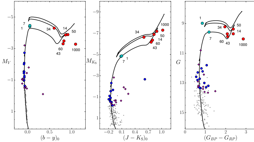
Fig. 12. Colour-magnitude diagrams for likely members of NGC 2345 in three different photometric systems: Left : M_V/(b-y)_0 from the Strömgren photometry taken in this work; Center : M_{K_S}/(J-K_S)_0 (2MASS photometry) and Right : G/(G_{BP}-G_{RP}) ( Gaia DR2 data). Photometric data for likely members appear as grey dots. Stars observed spectroscopically are represented as red circles (RSGs), cyan circles (A supergiants), blue circles (blue stars), and magenta diamonds (Be stars). The black line shows the best-fitting PAR-SEC isochrone ( \log \tau = 7.75 ).
