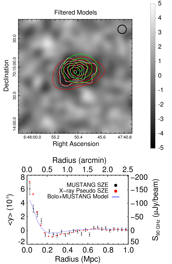
Figure 7. MACS J0647.7+7015 pseudo SZE map derived from Chandra X-ray data (top, red contours) with green contours representing the Bolo + MUSTANG gNFW _{\gamma=0.9} model from this work. The MUSTANG transfer function has been applied to both and the MUSTANG PSF is shown as a black circle. The white contours are MUSTANG S/N from Figure 4. The red and green contours are overlaid in units of -50 \mu\text{Jy beam}^{-1} starting at -50 \mu\text{Jy beam}^{-1} . Azimuthally averaged radial profiles are shown in the lower panel. Aside from the central \sim 0.1 Mpc where the X-ray and SZE flux are sharply peaked, the radially averaged flux from MUSTANG closely follows both the gNFW _{\gamma=0.9} model and the X-ray pseudo SZE flux.
