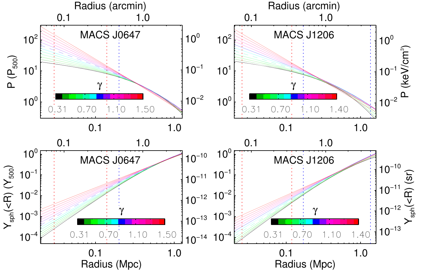
Figure 2. Pressure (upper) and spherically integrated Compton- y (lower) profiles generated from fits of generalized NFW profiles to Bolocam measurements of MACS J0647.7+7015 and MACS J1206.2–0847, in the left and right columns, respectively. Each profile represents the gNFW that best fits the Bolocam data given a fixed value of \gamma , represented by the color bars, with \alpha and \beta held at the A10 values. In general, Bolocam has the largest constraining power between 1' and 3' in radius, and all of the models overlap to a high degree in this radial region. This highlights the inherent parameter degeneracies between P_0 , R_s , and \gamma in the gNFW model, which can be broken using the high-resolution MUSTANG data. The dashed lines correspond to the best fit Bolo+MUSTANG models, which have \gamma = 0.9 for MACS J0647.7+7015, and \gamma = 0.7 for MACS J1206.2–0847 (see Table 3). From left to right, the vertical dotted lines mark the resolution and FOV, respectively, of MUSTANG (red) and Bolocam (blue), as in Figure 1.
