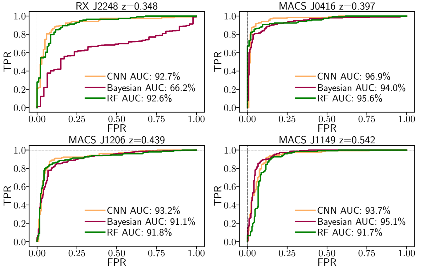
Fig. D.3. Comparison between the image-based CNN and two photometric catalogue-based approaches, RF and Bayesian method ( EXP3 ) in terms of ROC curves for the four clusters: R2248 (top-left panel), M0416 (top-right panel), M1206 (bottom left panel), M1149 (bottom right panel).
