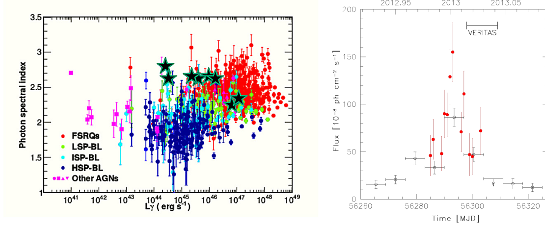
Figure 1. (Left panel): Photon index versus \gamma -ray luminosity of different types of Active Galactic Nuclei (AGN) included in the 3LAC. Black stars represent the values obtained over 7 years for narrow-line Seyfert 1 (NLSy1). Adapted from [20]; (Right panel): LAT light curve of PMN J0948+0022 in the 0.1–100 GeV energy range during 1 December 2012–31 January 2013 with 7-day time bins. Arrow refers to 2\sigma upper limit. Upper limits are computed when TS < 10 . Red solid circles represent daily fluxes reported for the periods of high activity. The horizontal line indicates the period of the VERITAS observation. Adapted from [13].
