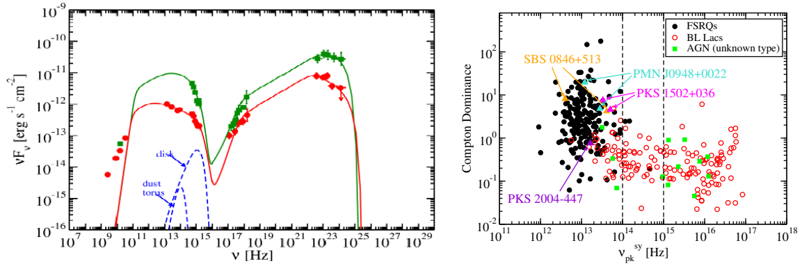
Figure 2. (Left panel): Spectral energy distribution (SED) and model fit (solid curve) of SBS 0846+513 in flaring activity (squares) and low activity (circles) with the disk and dust torus emission components shown as dashed curves. Adapted from [21]; (Right panel): the Compton dominance versus peak synchrotron frequency for sources from the Second LAT AGN catalog (2LAC) [53], along with two activity states of SBS 0846+513 [21], PMN J0948+0022 [23], PKS 1502+036 [25], and an average state of PKS 2004–447 [31]. Dashed lines indicate the boundary between high-synchrotron-peak, intermediate-synchrotron-peaked, and low-synchrotron-peaked blazars. Adapted from [54], reproduced by permission of the AAS.
