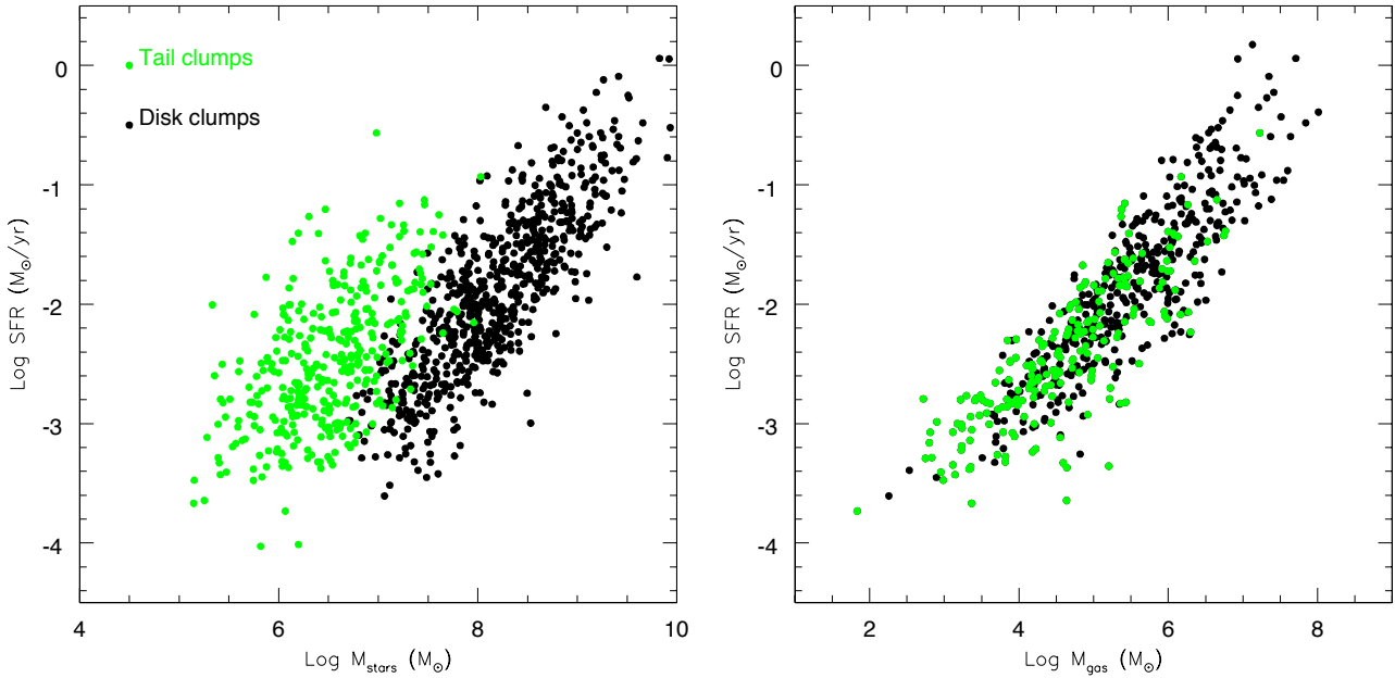
Figure 11. SFR-stellar mass (left) and SFR-gas mass (right) relations of clumps in the tails (green) and in the disks (black).
