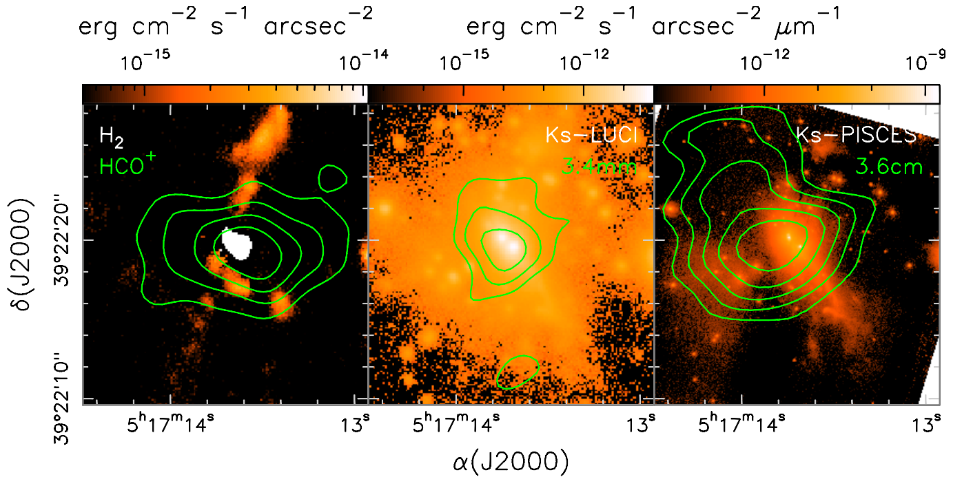
Fig. 13. Left: overlay of the contour map of the HCO + (1-0) line (from Molinari et al. 2002) obtained by averaging the emission between -27.08 and -23.72 \text{ km s}^{-1} , on the H 2 line (i.e. continuum subtracted) LUCI image. Contour levels range from 150 to 420 in steps of 90 mJy/beam. Like in Fig. 12, the area around stars A1, A2, and B has been blanked to mask an artefact caused by the continuum-subtraction process. Middle: overlay of the contour map of the 3.4 mm continuum emission (from Molinari et al. 2002) on the 2.2 \mu\text{m} continuum LUCI image. Contour levels range from 2.64 to 4.4 in steps of 0.88 mJy/beam. Right: overlay of the contour map of the 3.6 cm continuum emission (from Molinari et al. 2002) on the 2.2 \mu\text{m} continuum PISCES image. Contour levels range from 0.069 to 0.161 in steps of 0.023 mJy/beam.
