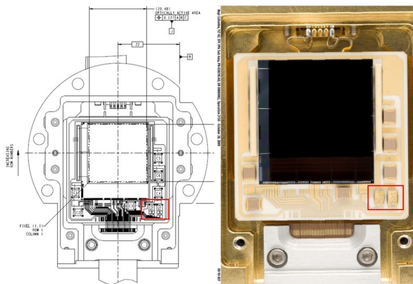
Figure 1 HRIC-FPA temperature sensors [RD2] Channel next to the FPA, called SCA1 (on the left) and SCA2 (on the right) and associated respectively to the NSS11040 and NSS11041.
