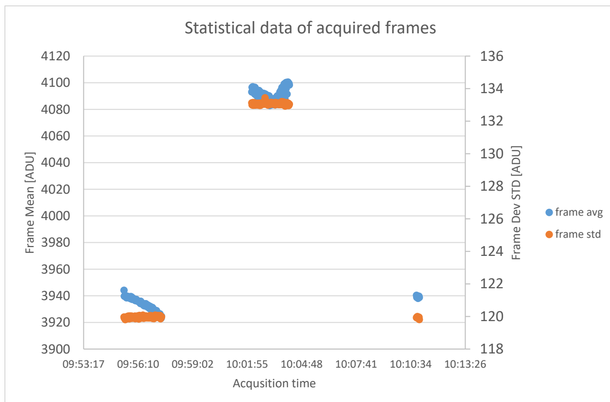
Figure 3 In the plot are reported the average and the standard deviation over the whole frame for the pixel readings. The frames have been acquired in three steps changing the integration time: a) short integration time .000038 s; b) long integration time 0.3148 s; c) short integration time 0.000038 s.
