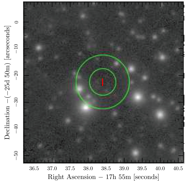
Figure 9. The stacked Pan-STARRS data in y band. The circles indicate 5 and 10 arcsec radius around the position of PSR J1755–2550 from radio timing. The red rectangle shows the uncertainty of position from radio timing.
