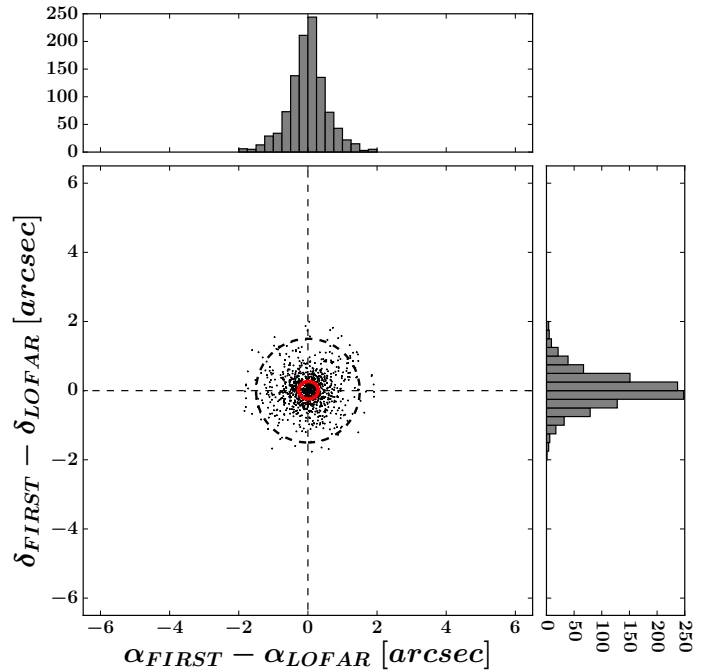
Fig. 8. Corrected positional offsets between high S/N and compact LOFAR sources and their FIRST counterparts (see text for more details). The dashed lines denotes a circle with radius r = 1.5'' , which is the image pixel scale. The ellipse (red solid line) centered on the right ascension and declination mean offsets indicates the standard deviation for both directions.
