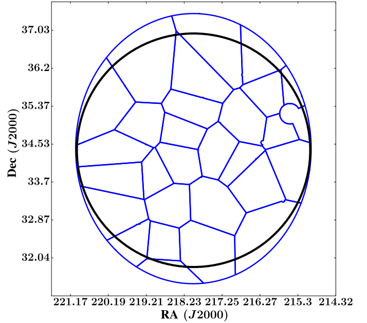
Fig. 2. The spatial distribution of the facets in the Boötes field (blue solid lines). The large circle (solid black line) indicates the radial cutoff of 2.5^\circ used to apply the primary beam correction.
