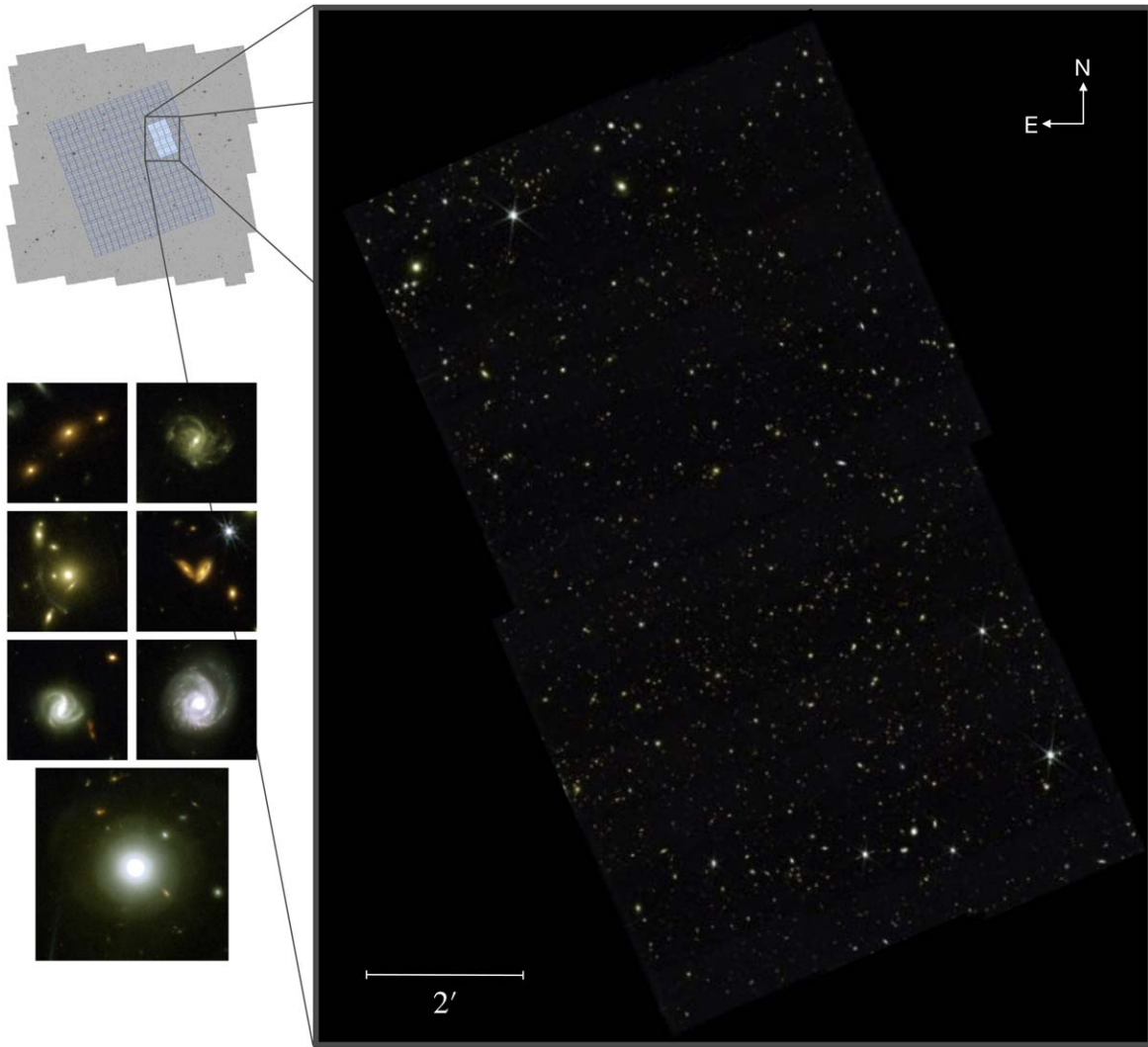
Figure 6. The first epoch of COSMOS-Web NIRC2 observations obtained on 2023 January 5–6. These data cover six visits (or pointings) out of a total of 152. The total area covered by NIRC2 here is \sim 77 arcmin 2 . The relative position of this mosaic in the survey is shown at upper left. At lower left are several zoomed-in 10'' \times 10'' cutouts (and one 16'' \times 16'' cutout) of a handful of interesting objects, highlighting the level of detail revealed by these first data.
