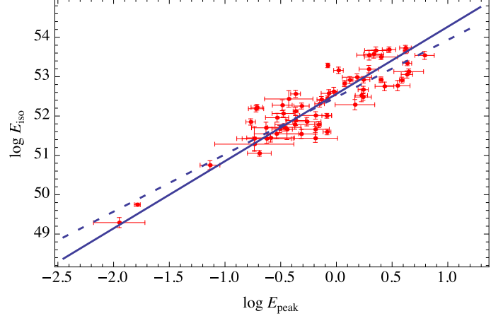
Fig. 2. Best-fit curves for the E_{p,i} - E_{iso} correlation relation superimposed on the data. The solid and dashed lines refer to the results obtained with the maximum likelihood (Reichart likelihood) and weighted \chi^2 estimator, respectively.
