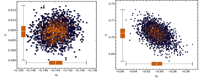
Fig. 5. Confidence regions in the (q_0 - j_0) plane, as provided by Cosmography Ib and II. The inner brown region defines the 2\sigma confidence level. The parameters q_0 and j_0 are well constrained, the values q_0 > 0 are ruled out, the value j_0 = 1 (which is the \Lambda CDM value) is statistically not favorable. On the axes we also plot the box-and-whisker diagrams for the respective parameters: the bottom and top of the diagrams are the 25th and 75th percentile (the lower and upper quartiles, respectively), and the band near the middle of the box is the median.
