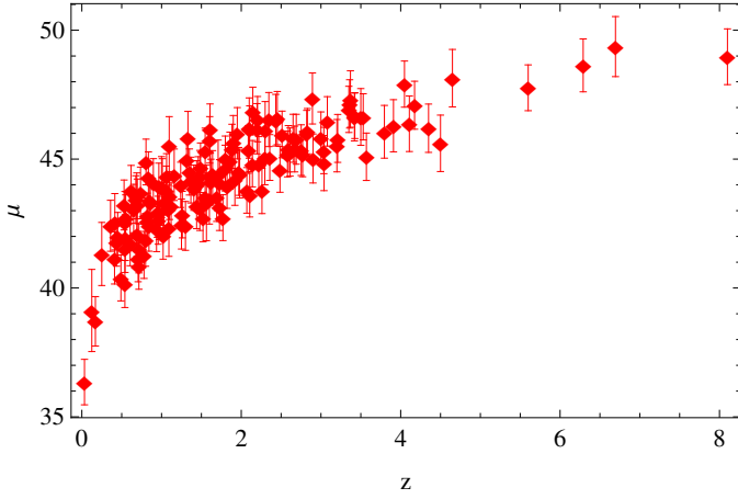
Fig. 3. Distance modulus \mu(z) for the calibrated GRB Hubble diagram obtained by fitting the E_{p,i} - E_{iso} relation.
