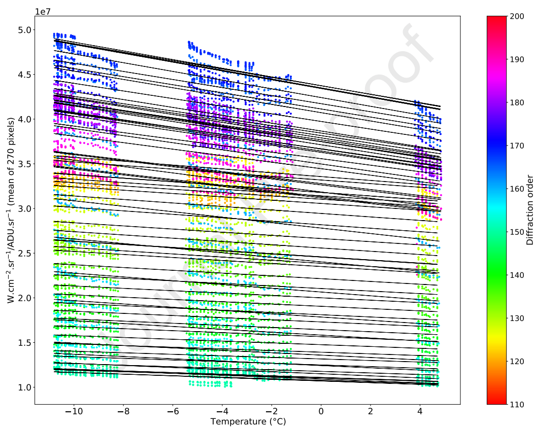
Figure 9: Sensitivity as a function of the instrumental temperature (nominal sensor). The colors refer to diffraction order and the dotted line shows the linear regression per order.
