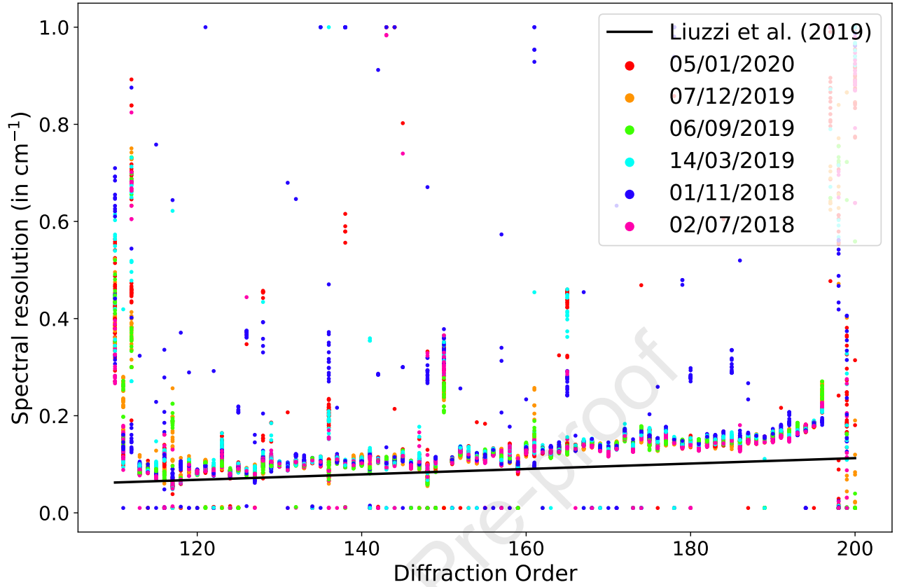
Figure 12: Actual ILS spectral resolution \sigma_\nu retrieved from the calibration inversion. Each point corresponds to a single spectrum, the color refers to the 6 fullscans used. The empirical spectral resolution computed using eq. 15 (Liuzzi et al., 2019)) is shown as a black line. For a clearer comparison, data from Liuzzi et al. (2019) were converted from a Gaussian FWHM to a Gaussian standard deviation considering FWHM = 2\sqrt{2\ln 2}\sigma
