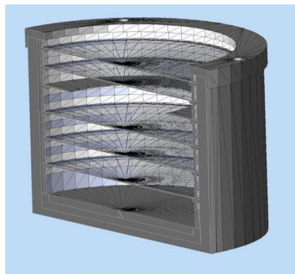
Figure 1: PA sketch. Internal layers represent the particle selection grids
