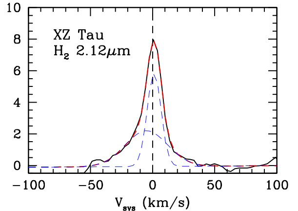
Fig. 13. Profile of the H 2 2.12 \mu\text{m} line detected in XZ Tau with the fit of the two Gaussian components superimposed. The red-dashed line is the best fit obtained by the sum of the two Gaussian components plotted as blue-dashed lines. Parameters of the two components are given in Table 2.
