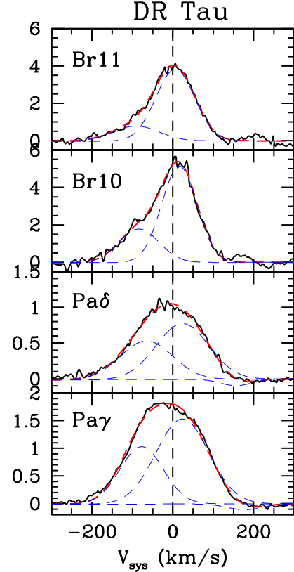
Fig. 7. The profile of bright H I lines in DR Tau is deconvolved with two Gaussians, one centred close to systemic velocity and the other blue-shifted at V_{\text{sys}} \sim -70/-100 km s ^{-1} .
