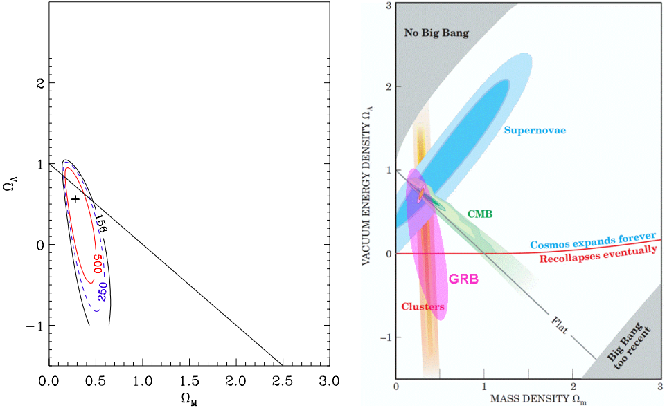
Fig. 6. (Color online) Left: 68% c.l. contour in the \Omega_M-\Omega_\Lambda plane obtained by releasing the flat universe assumption with the sample of 156 GRBs available at the end of 2012 (black) compared to those expected in the next years with the increasing of GRBs in the sample (blue and red). 41 Right: 68% c.l. contour in the \Omega_M-\Omega_\Lambda plane obtained by assuming a sample of 250 GRBs expected in the near future (pink) compared to those from other cosmological probes (adapted from a figure by the Supernova Cosmology Project 72 ).
