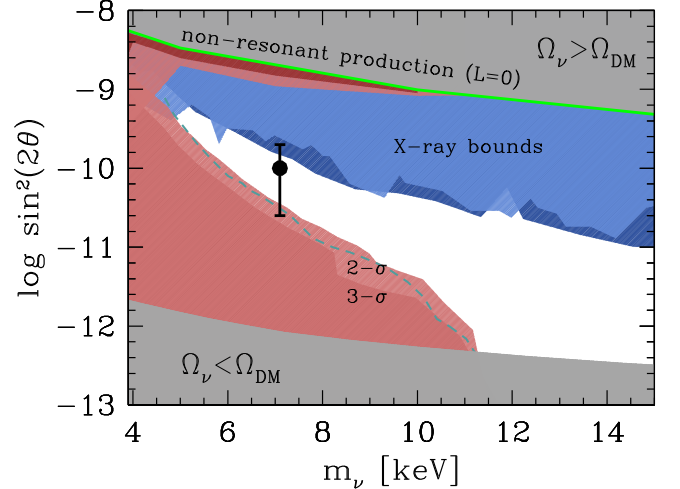
Figure 2. Constraints on the RP sterile neutrino parameter space from our method are represented as exclusion regions, with 3- \sigma and 2- \sigma limits represented by darker and lighter colors. Our constraints are compared with upper bounds from X-ray observations (as reported in Riemer-Sørensen 2016) of the Milky Way and dwarf galaxies. Gray areas are excluded by current limits on the abundance of DM (Ade et al. 2016). The green line corresponds to the non-resonant DW case with vanishing lepton asymmetry L = 0 . We also show as a dashed line the constraint obtained in Schneider (2016) from the abundance of satellites in the Milky Way. The tentative line signal at 7.1 keV (Boyarsky et al. 2014; Bulbul et al. 2014) is shown by the point with errorbars.
