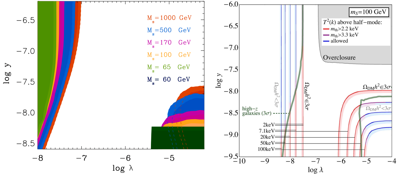
Figure 4. Left panel: the constraints on the parameter space of SD production model for sterile neutrinos. The colored regions represent the allowed region ( \bar{\phi} \geq \phi_{\text{obs}} ) in the \log \lambda – \log y plane for each value of the scalar mass m_s (shown by different colors according to the labels on the right). For each scalar mass (and hence for each color) lighter and darker tonalities represent the 1- \sigma and 2- \sigma confidence levels, respectively. Right panel: for the case m_s = 100 GeV, we compare our bounds from HFF galaxies derived in the present work (green thick lines) with a version of Ly \alpha bounds derived by König et al. (2016): the latter are represented as red (forbidden cases), blue (allowed cases), and purple (constrained cases) segments in the lines of constant m_\nu values in the \log \lambda – \log y plane.
