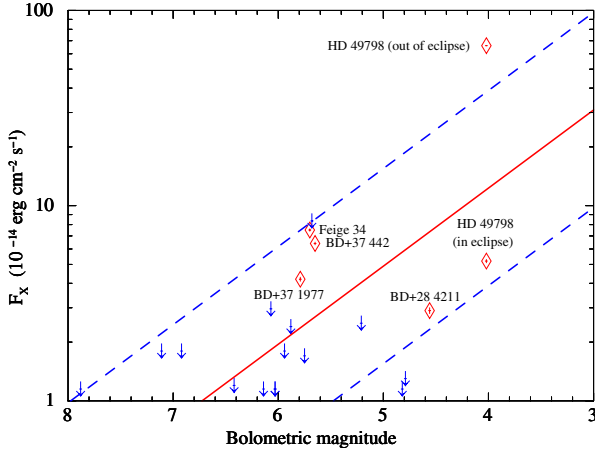
Fig. 5. Level of the X-ray flux (or its upper limit for the undetected sources) of the sdO stars observed at X-rays, as a function of their bolometric magnitude. The upper and lower blue lines (corresponding to f_X/f_{\text{bol}} = 10^{-6.2} and f_X/f_{\text{bol}} = 10^{-7.2} , respectively) include the range of expected values for the main-sequence early-type stars; the red line corresponds to f_X/f_{\text{bol}} = 10^{-6.7} , which is the best-fit relation found by Nazé (2009) for this type of stars.
