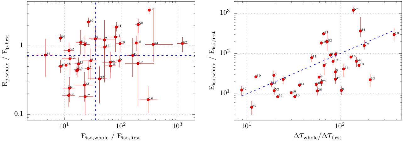
Figure 3. Left-hand panel: ratio of whole-to-first peak energy versus the same ratio for E_{iso} . The blue dashed lines are the median values of both ratios. Right-hand panel: the E_{iso,whole}/E_{iso,first} ratio versus \Delta T_{whole}/\Delta T_{first} . The blue dashed line is the 1:1 line. The numbers beside the symbols are the GRB identifiers shown in Tables A1 and A2.
