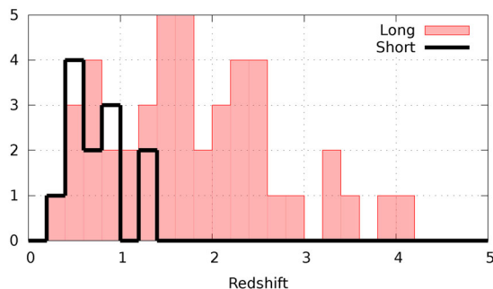
Figure 1. Redshift distribution for both the SGRB (12) and LGRB (45) bursts (references for redshift estimates are given in Table A1).
