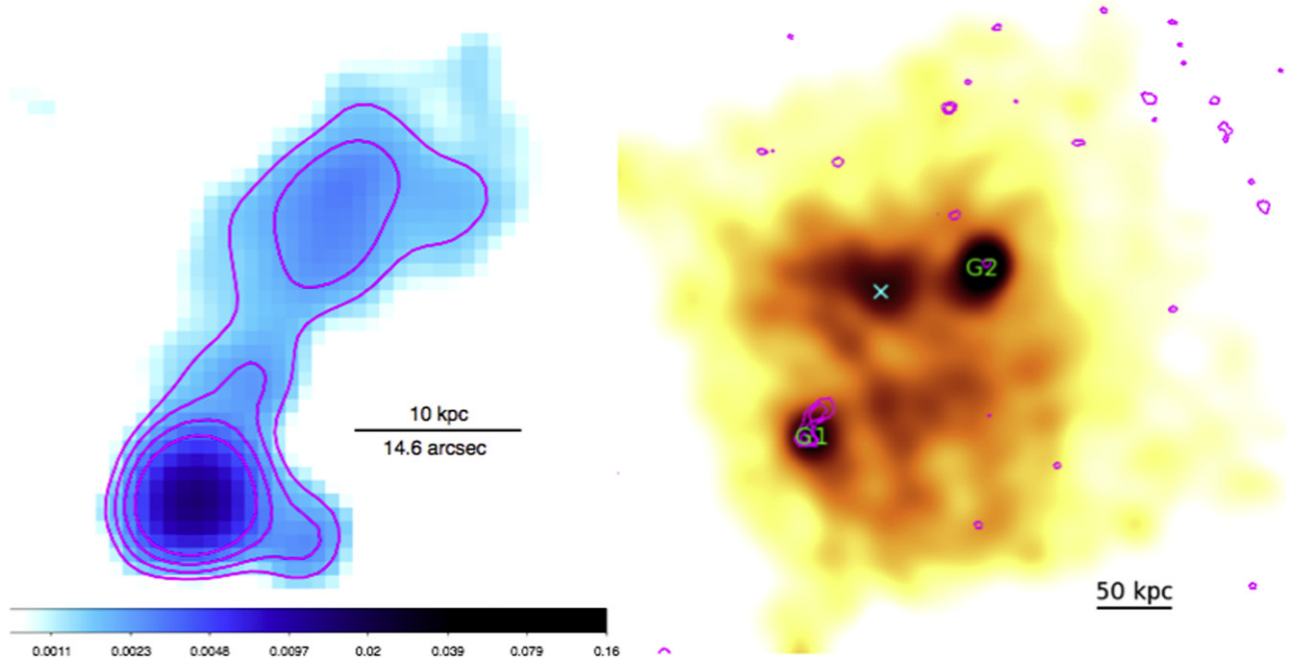
Figure 10. Left: VLA radio image of G1 showing extended radio emission in the northwest direction in units of \text{Jy beam}^{-1} . Magenta contour levels are set at \sqrt[4]{1, 2, 4, 8} \times 4\sigma_{\text{rms}} , where \sigma_{\text{rms}} = 0.37 \text{ mJy beam}^{-1} . Right: Chandra X-ray image of Abell 1142 with the radio contour overlaid.
