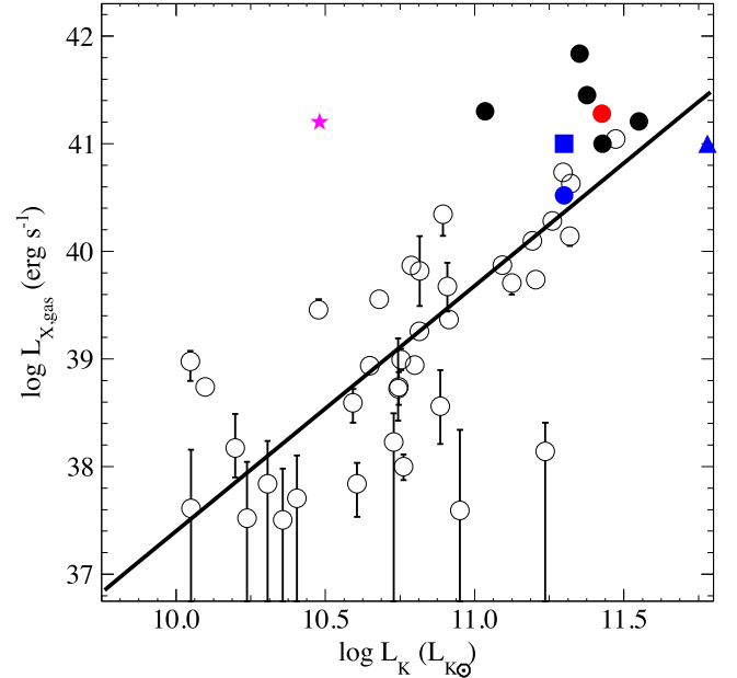
Figure 11. Gaseous X-ray luminosities as a function of K -band luminosities for all galaxies taken from Su et al. (2015b). The black solid line is the best-fit L_{X,\text{gas}}-L_K relation. Black solid circles indicate group center galaxies. Red circle represents IC 664 (G2). Blue symbols represent NGC 3492 (G1)—blue circle: using the average L_{X,\text{gas}} and L_K of the three galaxies in G1; blue square: assuming all the L_{X,\text{gas}} is from one of the three galaxies; blue triangle: treating all three galaxies as one galaxy (total L_{X,\text{gas}} and L_K ). Magenta star represents the small galaxy at the central X-ray peak.
