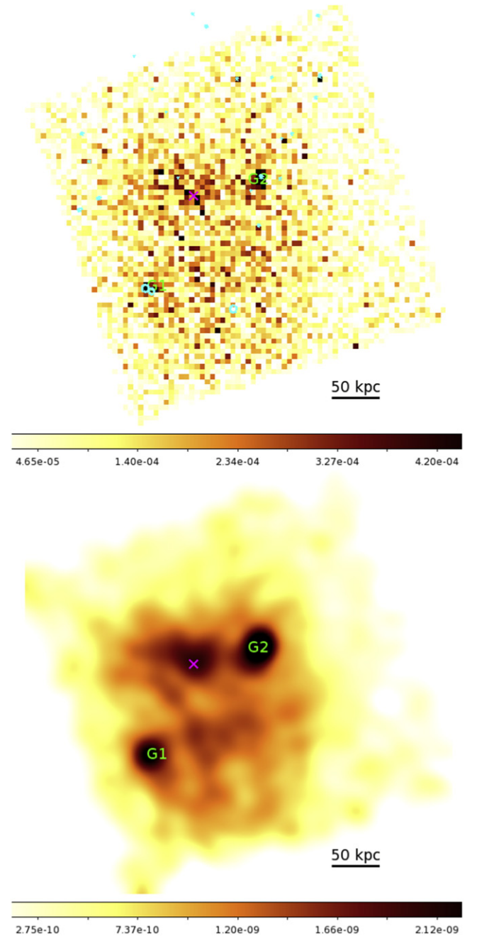
Figure 1. 27 ks exposure-corrected and blank-sky background subtracted Chandra ACIS-S image of Abell 1142 and in the energy band of 0.5–4.0 keV. Top: the image was binned by 16 \times 16 pixels in units of counts \text{s}^{-1} . Positions of point sources were marked in cyan ellipsicals. Bottom: adaptively smoothed in units of photon \text{cm}^{-2} \text{s}^{-1} . Locations of G1 and G2 are indicated. The peak of cluster gas emission is indicated by the magenta cross.
