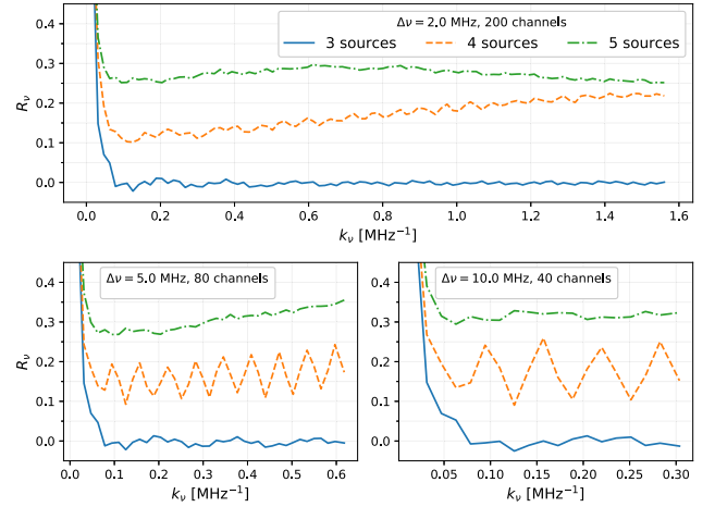
Figure 8. Relative difference in radial power spectrum between the GMCA recovered signal and the input cosmological signal and instrumental noise. The three different simulations (panels) are full-sky and GMCA has been run with number of sources n_s = 3, 4 , and 5 (solid, dashed, and dash-dotted lines, respectively). These simulations lack the polarization leakage contribution. GMCA recovers unbiased information in the radial direction for k_v \gtrsim 0.05 \text{ MHz}^{-1} when n_s = 3 is set.
