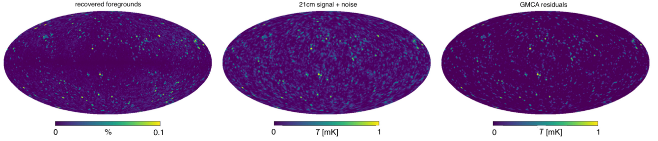
Figure 6. Foreground removal for the \nu \in [1100\text{--}1102] MHz channel, GMCA has looked for n_s = 3 components. Left-hand map: relative difference in percentage between the input foregrounds, \mathbf{F} , and what found by GMCA, \mathbf{X}^{\text{GMCA}} . Middle map: input 21-cm signal and instrumental noise, \mathbf{C} + \mathbf{N} . Right-hand map: foreground removal residuals \mathbf{X}^{\text{cleaned}} , to be compared with middle map. Foregrounds total temperature is recovered at sub-per cent level, especially in the galactic plane, yet we miss some of the low-temperature features of the input signal map; the brightest 21-cm spots are recovered in the map in the right, and they also represent the regions at most off-set in the foreground recovery (left).
