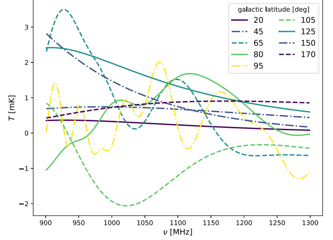
Figure 2. Temperature contribution of the polarization leakage as function of frequency, observed along different lines of sight at constant galactic longitude but different latitudes. The leakage has a smooth behaviour at the poles – although dependent on line of sight – and oscillates when closer to the galactic plane.
