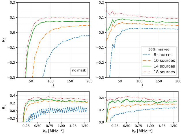
Figure 14. Relative difference in power spectrum between the GMCA recovered signal and the input cosmological signal and instrumental noise: angular R_\ell (radial R_v ) in the top (bottom) row. GMCA has been run on the data cube that also contains a 0.5 per cent polarization leaked into the unpolarized signal. On the left-hand panel, we consider the full-sky maps, on the right 50 per cent of the maps have been masked out. Different line styles and colours correspond to different number of components n_s = 6, 10, 14 , and 18 GMCA has been run with. When excluding the galactic plane region (right-hand panel), GMCA reconstructions improve. Anyway, also for the full-sky scenarios in left-hand panel, results are encouraging at small scales.
