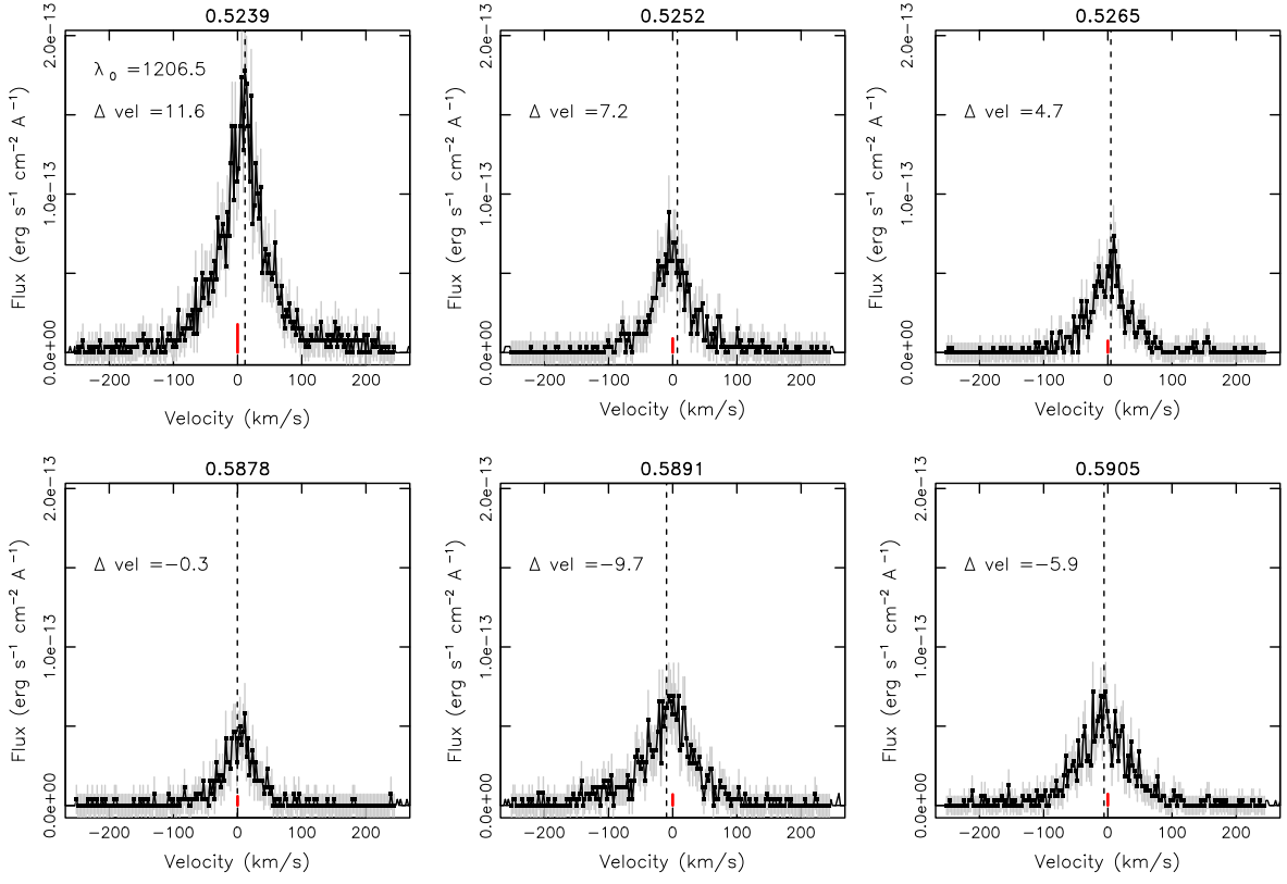
Figure 15. Same as in Figure 13 for the Si III line at 1206.5 Å.
