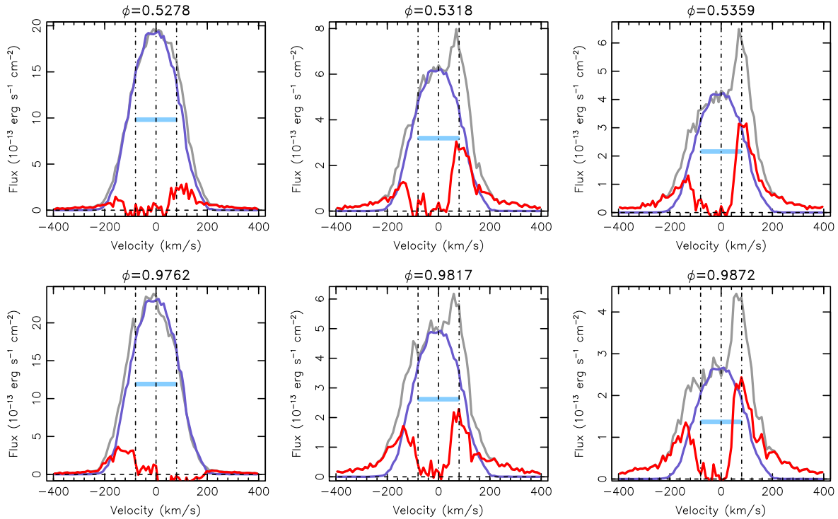
Figure 11. Examples of Ly \alpha profiles corrected for the air-glow emission in Doppler-shift velocity space. The orbital planetary phase is indicated on the top of each panel. The gray line is the raw profile, blue is the air-glow contamination, and red line is the corrected profile. Vertical lines mark the rest position and \pm 80 km s ^{-1} . The expected width of the uncontaminated and unabsorbed Ly \alpha (150 km s ^{-1} ) is shown with the light-blue horizontal bar.
