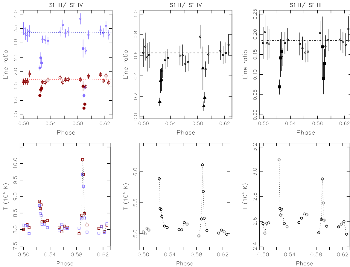
Figure 6. Top row: ratio of Si lines as a function of the planetary orbital phase. Filled symbols are the points from subinterval spectra. Left panel: Si III/ Si IV 1402.5 Å (blue symbols), Si III/ Si IV 1393.7 Å (red symbols). Central panel: Si II/ Si IV 1402.5 Å. Right panel: Si II/ Si III. Bottom row: temperature versus planetary phase derived from the line ratios. The comparison of the two peaks shows that the second brightening was hotter in temperature than the first one.
