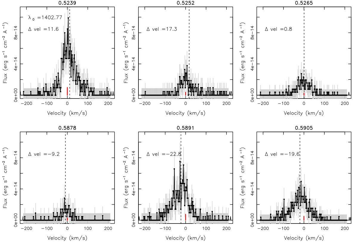
Figure 14. Same as in Figure 13 for the Si iv line at 1402.8 Å.
