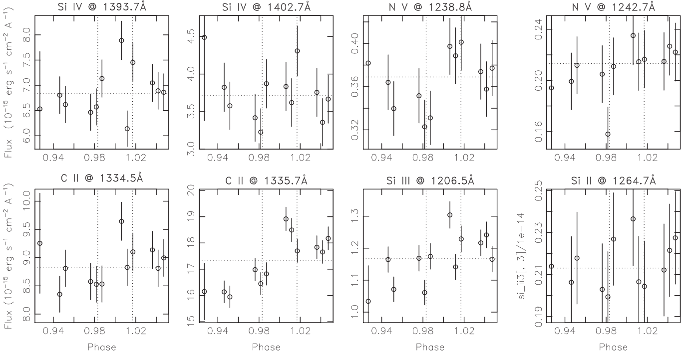
Figure 4. As in Figure 3, fluxes of lines as a function of the planetary phases from archival spectra obtained at the planetary transit. The names of lines are indicated on the top axis. The horizontal line represents the average stellar flux. Variability is observed at the \leq 3\sigma level only.
