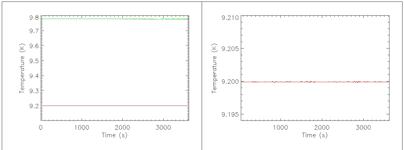
Figure 8-2: Left – Sky Load: (SKY_TEMP) probe (red) and (SMON_TMP) probe (green) temperature behaviour during the RCA_THF test; right – Ref Load (REF_TEMP) probe
